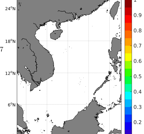
Temporal STD of (Sat-TSG-SAMOS) in 1°x1° boxes over -
