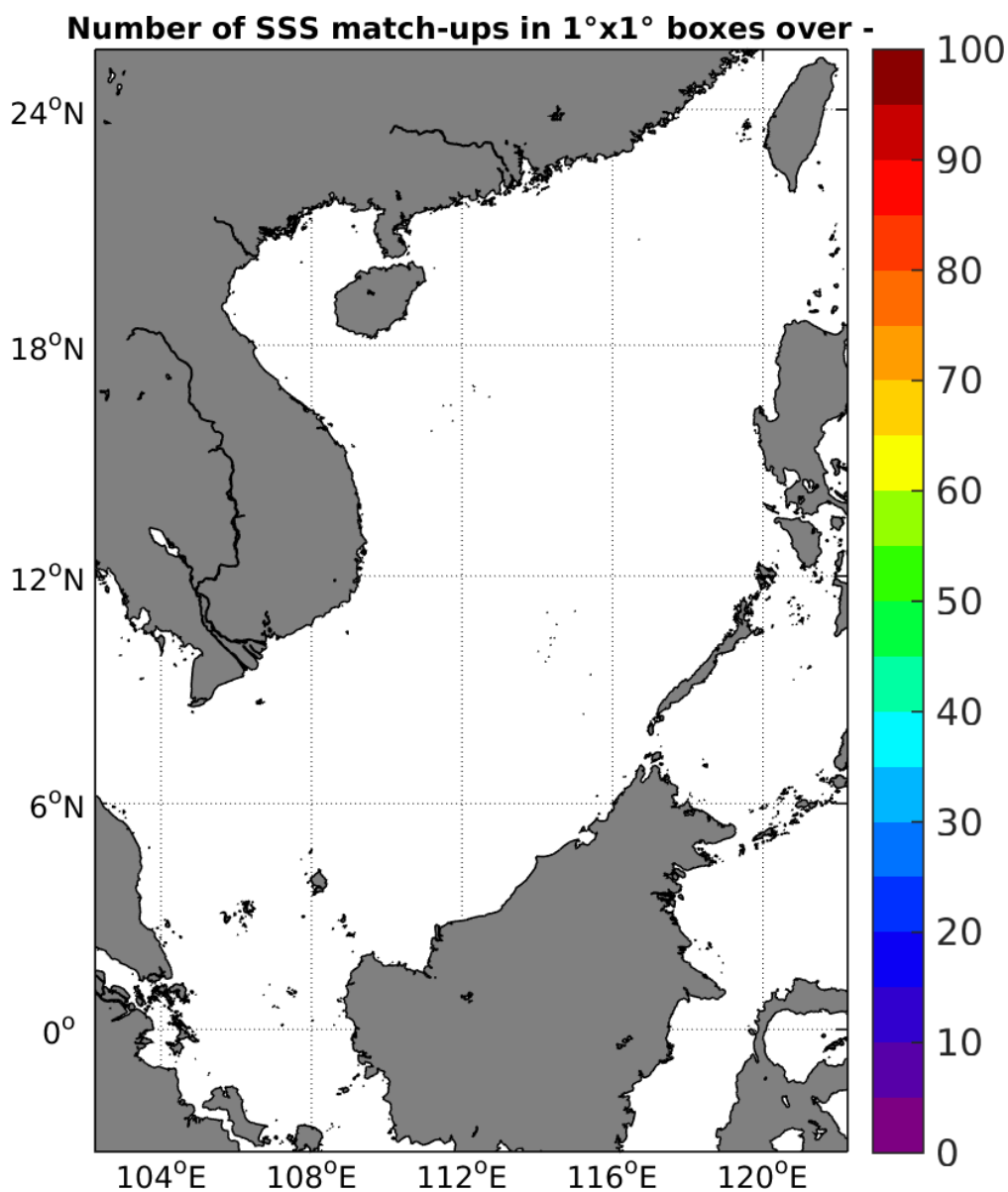
Figure 4: Number of SSS match-ups between TSG-SAMOS SSS and the AQUARIUS-L2-JPL-V4 SSS product for the South China Sea Pi-MEP region over 1°x1° boxes and for the full satellite product period.
