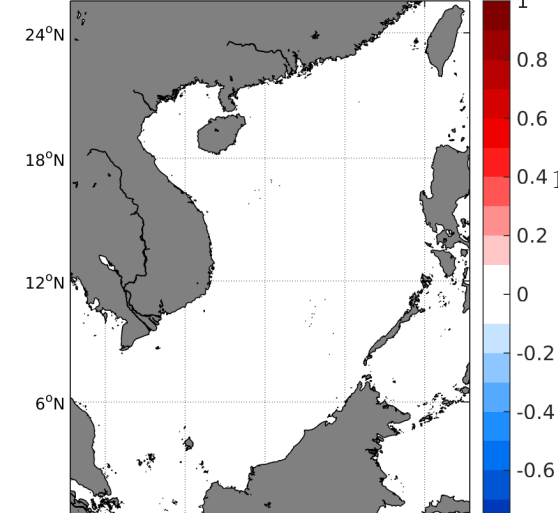
Temporal mean of (Sat-TSG-SAMOS) in 1°x1° boxes over -
