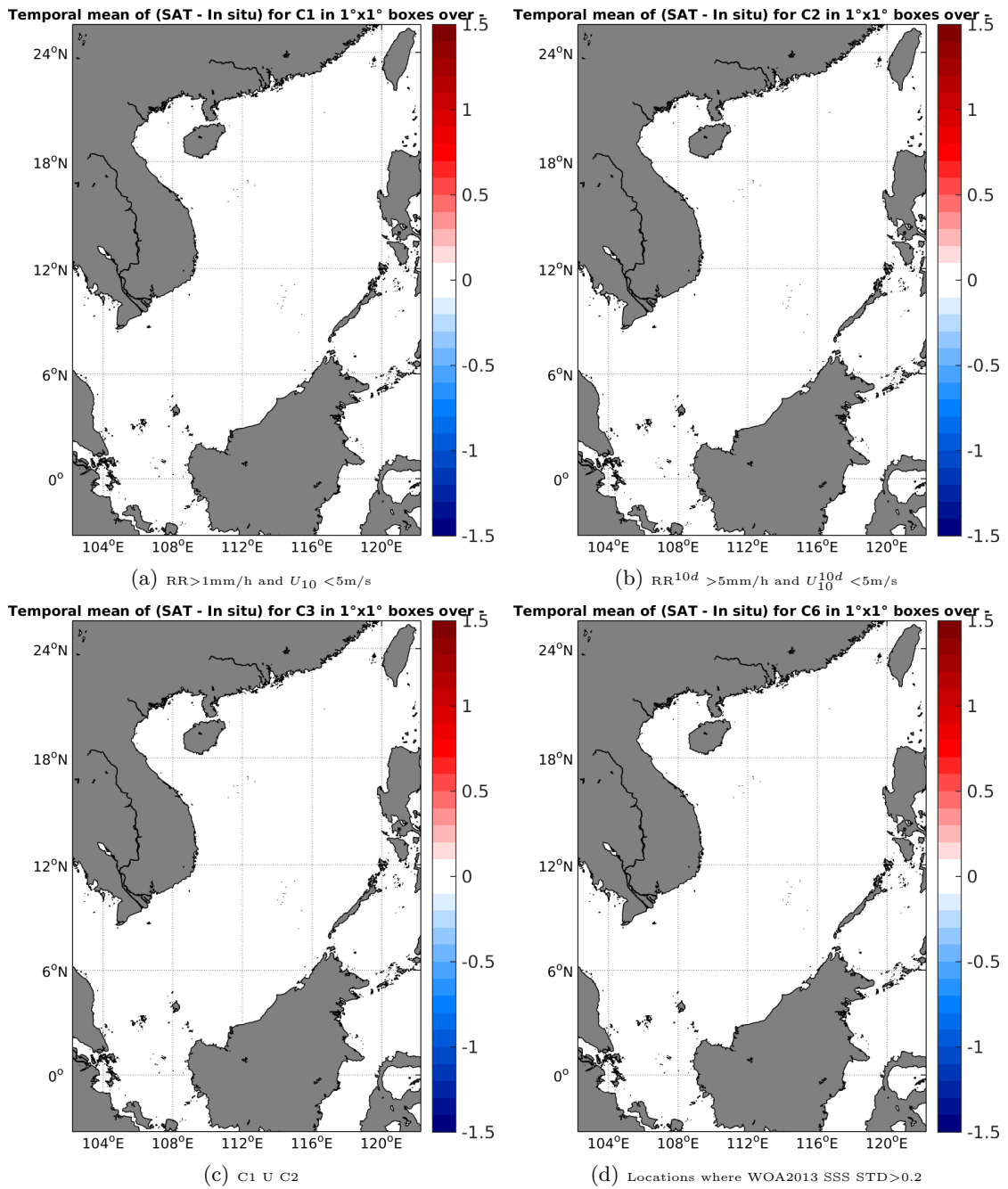
Figure 12: Temporal mean gridded over spatial boxes of size 1°x1° of \Delta\text{SSS} (AQUARIUS-L2-JPL-V4 - TSG-SAMOS) for 4 different subdatasets corresponding to: RR > 1\text{mm/h} and U_{10} < 5\text{m/s} (a), RR^{10d} > 5\text{mm/h} and U_{10}^{10d} < 5\text{m/s} (b), C1 U C2 (c), Locations where WOA2013 SSS STD > 0.2 (d).
