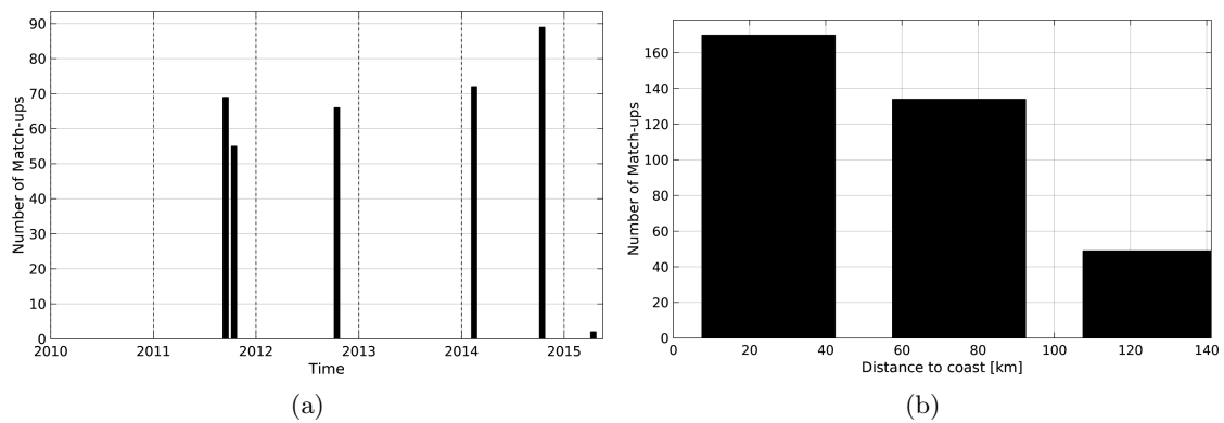
Figure 1: Number of match-ups between TSG-LEGOS-DM and AQUARIUS-L2-JPL-V4 SSS as a function of time (a) and as function of the distance to coast (b) over the South China Sea Pi-MEP region and for the full satellite product period.
