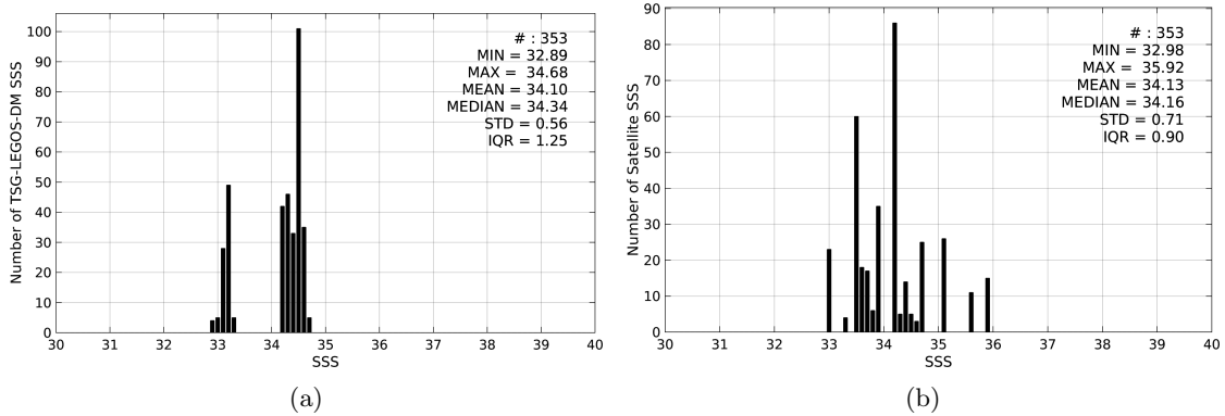
Figure 2: Histograms of SSS from TSG-LEGOS-DM (a) and AQUARIUS-L2-JPL-V4 (b) considering all match-up pairs per bins of 0.1 over the South China Sea Pi-MEP region and for the full satellite product period.
