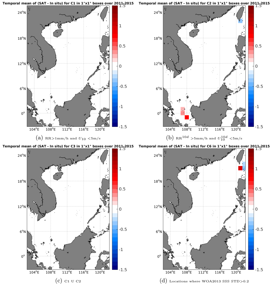
Figure 12: Temporal mean gridded over spatial boxes of size 1°x1° of \Delta SSS (AQUARIUS-L2-JPL-V4 - TSG-LEGOS-DM) for 4 different subdatasets corresponding to: RR > 1mm/h and U_{10} < 5 m/s (a), RR^{10d} > 5 mm/h and U_{10}^{10d} < 5 m/s (b), C1 U C2 (c), Locations where WOA2013 SSS STD > 0.2 (d).
