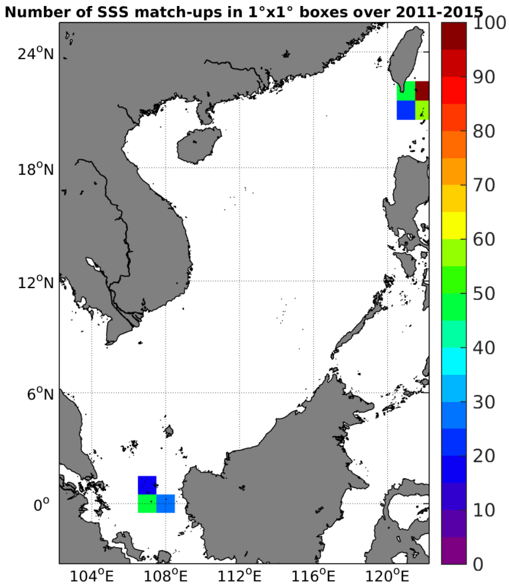
Figure 4: Number of SSS match-ups between TSG-LEGOS-DM SSS and the AQUARIUS-L2-JPL-V4 SSS product for the South China Sea Pi-MEP region over 1°x1° boxes and for the full satellite product period.
