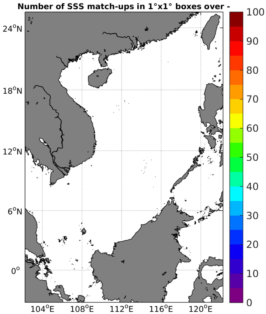
Figure 4: Number of SSS match-ups between TSG-GOSUD-Research-vessel SSS and the AQUARIUS-L2-JPL-V4 SSS product for the South China Sea Pi-MEP region over 1°x1° boxes and for the full satellite product period.
