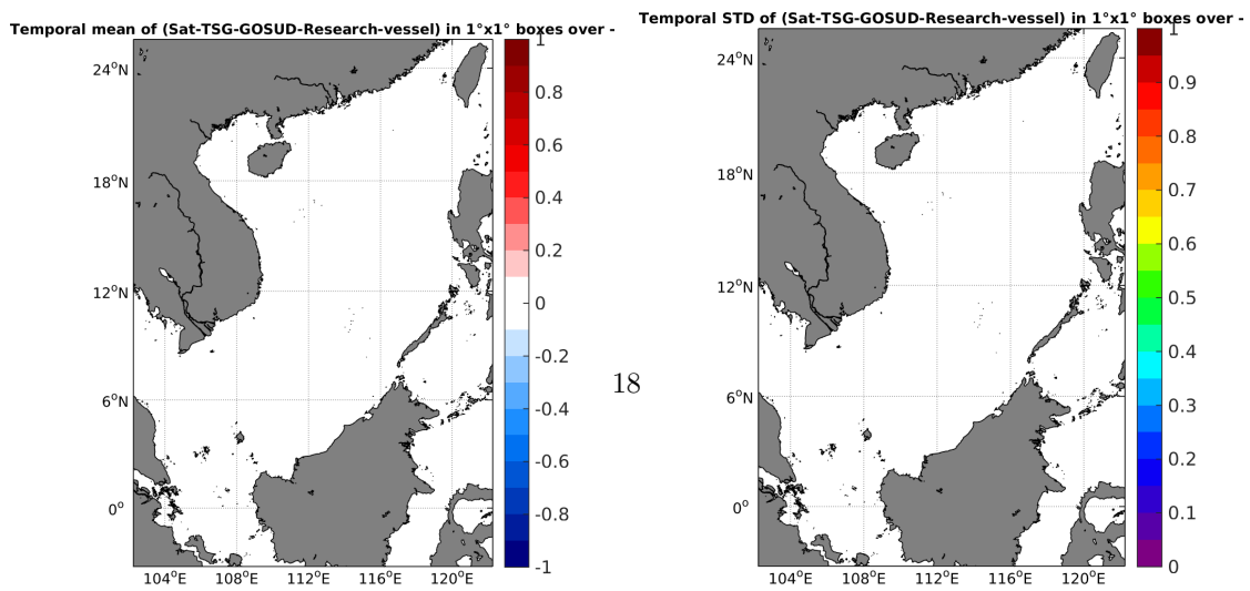
Figure 6: Temporal mean (left) and STD (right) of SSS from AQUARIUS-L2-JPL-V4 (top), TSG-GOSUD-Research-vessel (middle), and of \Delta SSS (Satellite - TSG-GOSUD-Research-vessel).
