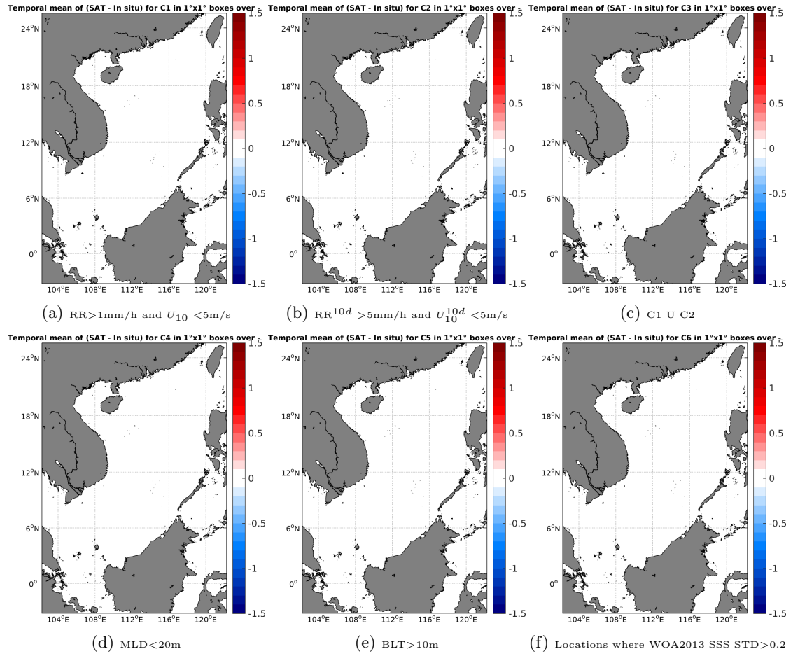
Figure 12: Temporal mean gridded over spatial boxes of size 1^\circ \times 1^\circ of \Delta SSS (AQUARIUS-L2-JPL-V4 - Sea mammals) for 6 different subdatasets corresponding to:RR>1mm/h and U_{10} < 5m/s (a), RR^{10d} > 5mm/h and U_{10}^{10d} < 5m/s (b), C1 U C2 (c),MLD<20m (d),BLT>10m (e),Locations where WOA2013 SSS STD>0.2 (f).
