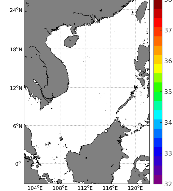
(c) MEAN(Sea mammals SSS)
