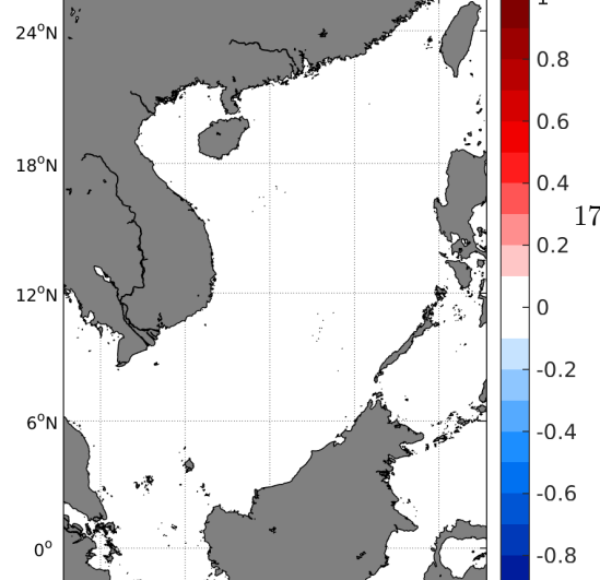
Temporal mean of (Sat-Surface drifters) in 1°x1° boxes over -
