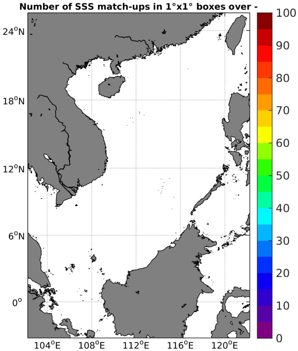
Figure 3: Number of SSS match-ups between Surface drifters SSS and the AQUARIUS-L2-JPL-V4 SSS product for the South China Sea Pi-MEP region over 1°x1° boxes and for the full satellite product period.
