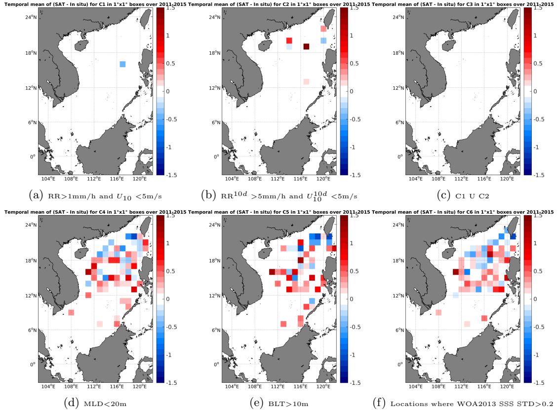
Figure 12: Temporal mean gridded over spatial boxes of size 1^\circ \times 1^\circ of \Delta SSS (AQUARIUS-L2-JPL-V4 - Argo) for 6 different subdatasets corresponding to:RR>1mm/h and U_{10} < 5\text{m/s} (a), RR^{10d} > 5\text{mm/h} and U_{10}^{10d} < 5\text{m/s} (b), C1 U C2 (c),MLD<20m (d),BLT>10m (e),Locations where WOA2013 SSS STD>0.2 (f).
