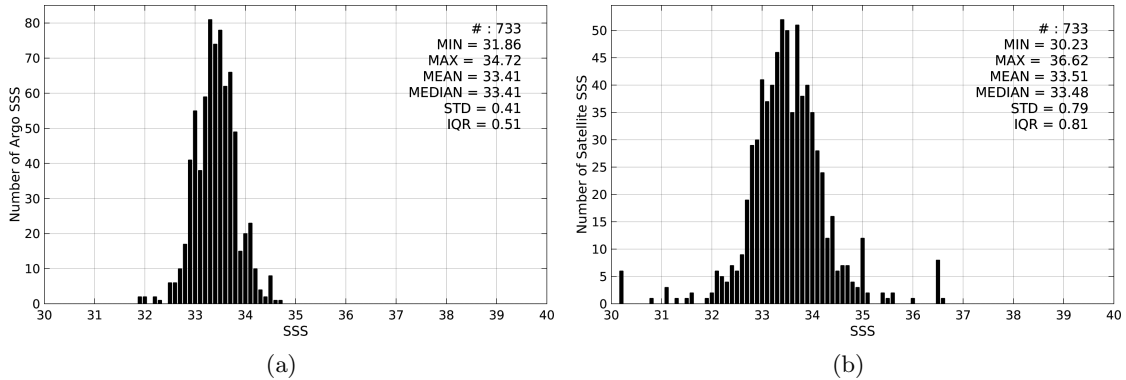
Figure 2: Histograms of SSS from Argo (a) and AQUARIUS-L2-JPL-V4 (b) considering all match-up pairs per bins of 0.1 over the South China Sea Pi-MEP region and for the full satellite product period.
