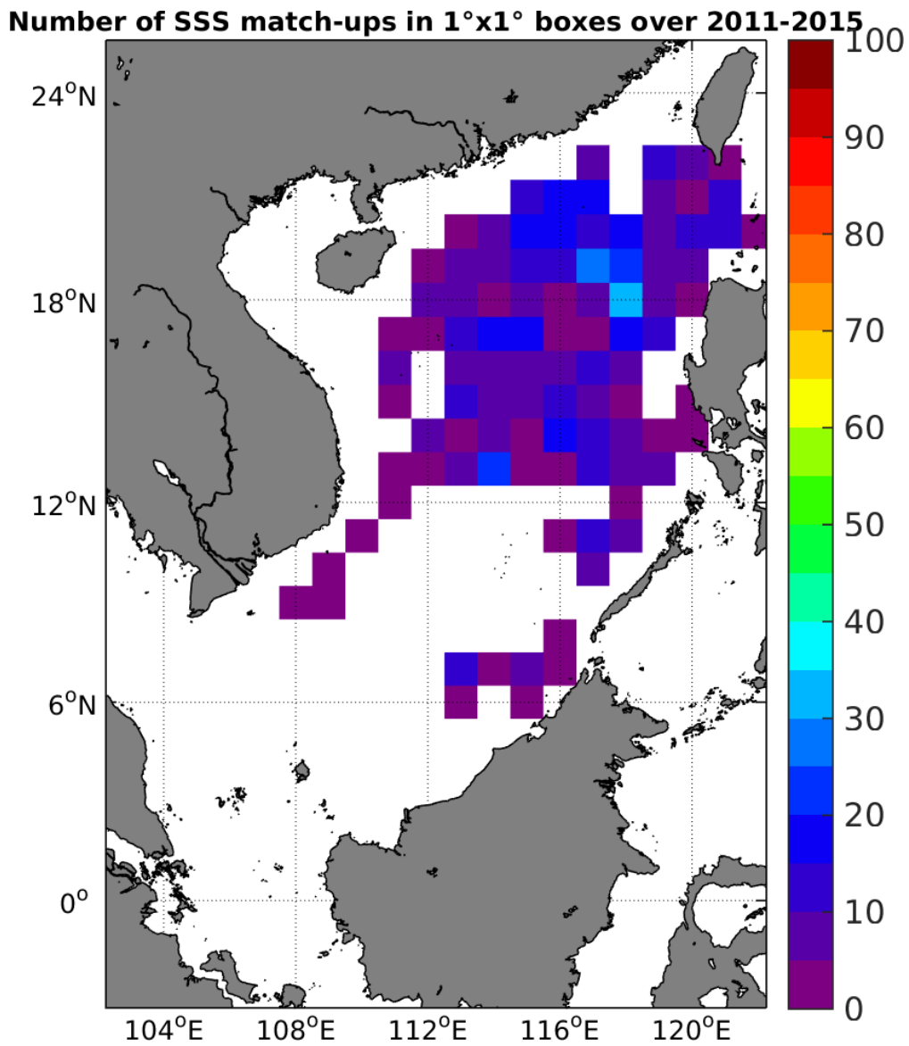
Figure 4: Number of SSS match-ups between Argo SSS and the AQUARIUS-L2-JPL-V4 SSS product for the South China Sea Pi-MEP region over 1°x1° boxes and for the full satellite product period.
