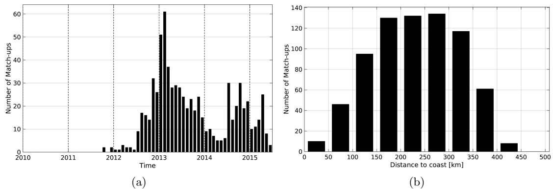
Figure 1: Number of match-ups between Argo and AQUARIUS-L2-JPL-V4 SSS as a function of time (a) and as function of the distance to coast (b) over the South China Sea Pi-MEP region and for the full satellite product period.
