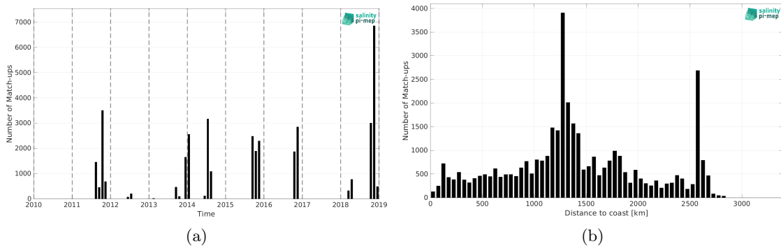
Figure 1: Number of match-ups between TSG (SAMOS) and SMOS and SMAP SSS L4 OI v1 - 7 Days (LOPS) SSS as a function of time (a) and as function of the distance to coast (b) over the South Atlantic Ocean Pi-MEP region and for the full satellite product period.
