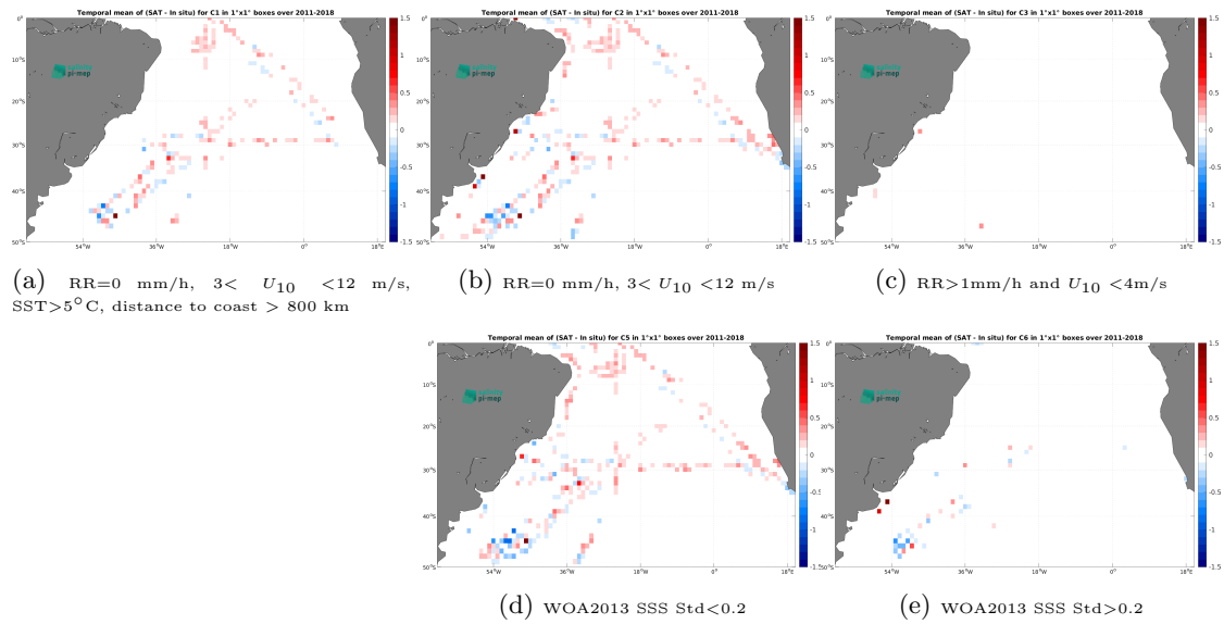
Figure 12: Temporal mean gridded over spatial boxes of size 1^\circ \times 1^\circ of \Delta\text{SSS} (SMOS and SMAP SSS L4 OI v1 - 7 Days (LOPS) - TSG (SAMOS)) for 5 different subdatasets corresponding to:RR=0 mm/h, 3 < U_{10} < 12 m/s, SST >5^\circ\text{C} , distance to coast > 800 km (a), RR=0 mm/h, 3 < U_{10} < 12 m/s (b), RR >1 mm/h and U_{10} < 4 m/s (c), WOA2013 SSS Std <0.2 (d), WOA2013 SSS Std >0.2 (e).
