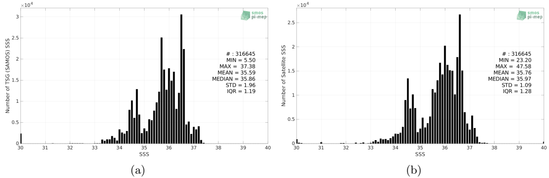
Figure 2: Histograms of SSS from TSG (SAMOS) (a) and SMOS and SMAP SSS L4 OI v1 - 7 Days (LOPS) (b) considering all match-up pairs per bins of 0.1 over the South Atlantic Ocean Pi-MEP region and for the full satellite product period.
