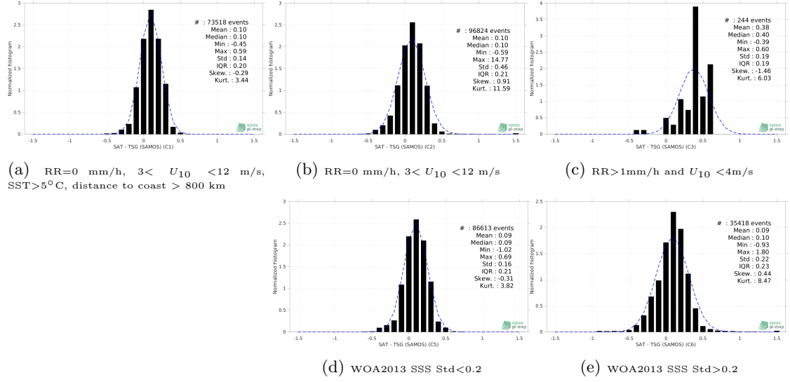
Figure 13: Normalized histogram of \Delta\text{SSS} (SMOS and SMAP SSS L4 OI v1 - 7 Days (LOPS) - TSG (SAMOS)) for 5 different subdatasets corresponding to: RR=0 mm/h, 3 < U_{10} < 12 m/s, SST>5°C, distance to coast > 800 km (a), RR=0 mm/h, 3 < U_{10} < 12 m/s (b), RR>1mm/h and U_{10} < 4 m/s (c), WOA2013 SSS Std<0.2 (d), WOA2013 SSS Std>0.2 (e).
