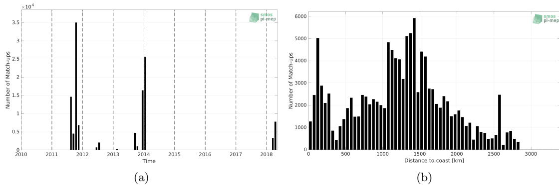
Figure 1: Number of match-ups between TSG (SAMOS) and SMOS and SMAP SSS L4 OI v1 - 7 Days (LOPS) SSS as a function of time (a) and as function of the distance to coast (b) over the South Atlantic Ocean Pi-MEP region and for the full satellite product period.
