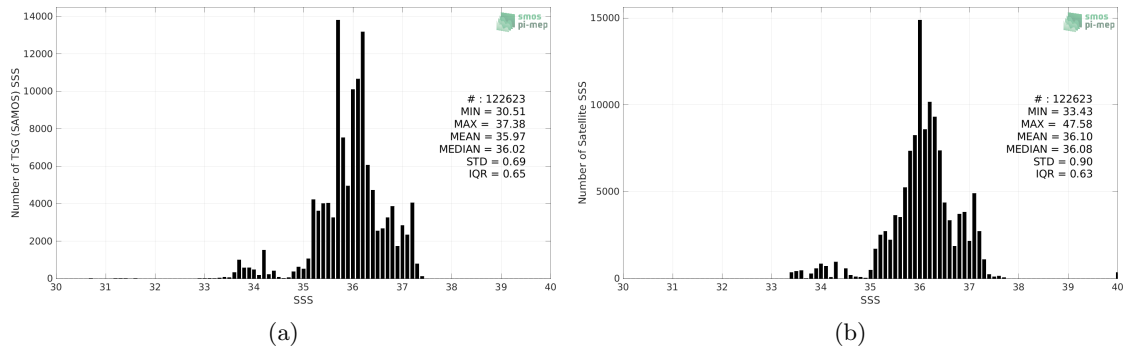
Figure 2: Histograms of SSS from TSG (SAMOS) (a) and SMOS and SMAP SSS L4 OI v1 - 7 Days (LOPS) (b) considering all match-up pairs per bins of 0.1 over the South Atlantic Ocean Pi-MEP region and for the full satellite product period.
