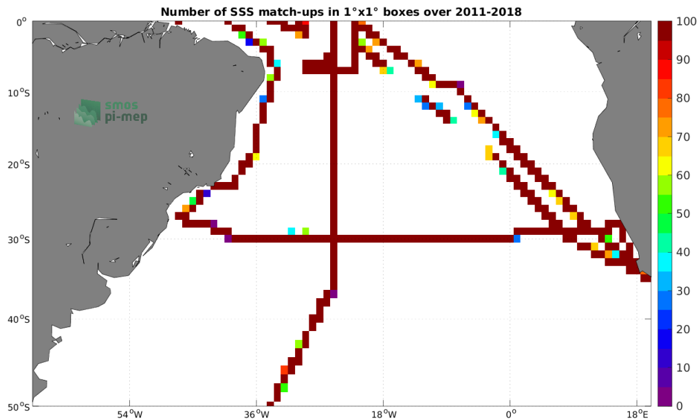
Figure 4: Number of SSS match-ups between TSG (SAMOS) SSS and the SMOS and SMAP SSS L4 OI v1 - 7 Days (LOPS) SSS product for the South Atlantic Ocean Pi-MEP region over 1^\circ \times 1^\circ boxes and for the full satellite product period.
