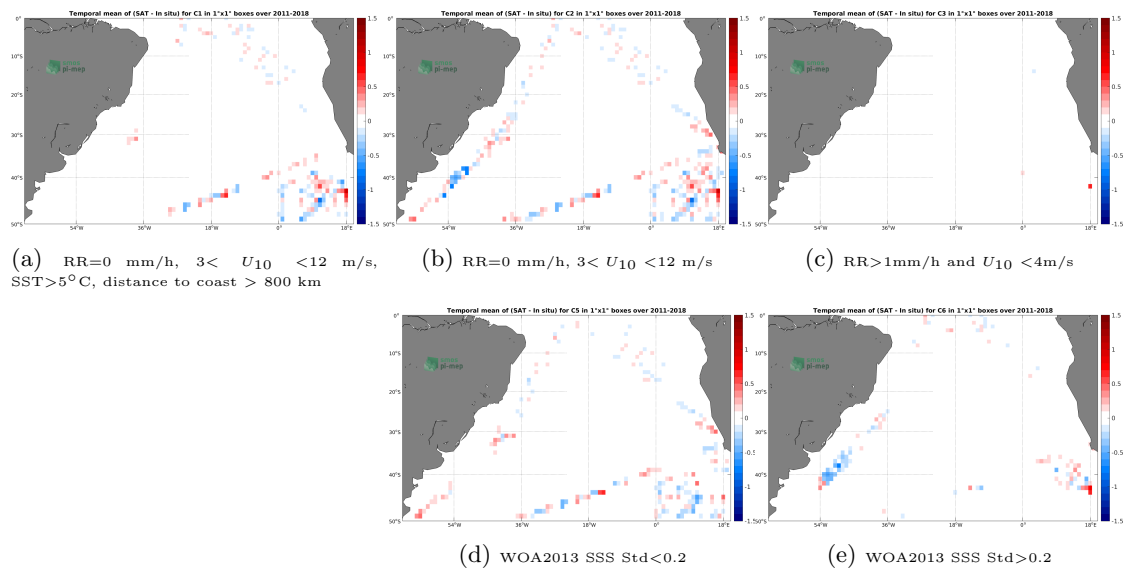
Figure 12: Temporal mean gridded over spatial boxes of size 1^\circ \times 1^\circ of \Delta SSS (SMOS and SMAP SSS L4 OI v1 - 7 Days (LOPS) - TSG (Polarstern)) for 5 different subdatasets corresponding to:RR=0 mm/h, 3 < U_{10} < 12 m/s, SST > 5^\circ\text{C} , distance to coast > 800 km (a), RR=0 mm/h, 3 < U_{10} < 12 m/s (b), RR > 1 mm/h and U_{10} < 4 m/s (c), WOA2013 SSS Std < 0.2 (d), WOA2013 SSS Std > 0.2 (e).
