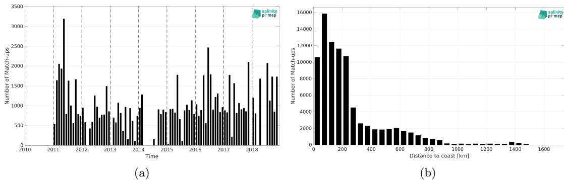
Figure 1: Number of match-ups between TSG (LEGOS-DM) and SMOS and SMAP SSS L4 OI v1 - 7 Days (LOPS) SSS as a function of time (a) and as function of the distance to coast (b) over the South Atlantic Ocean Pi-MEP region and for the full satellite product period.
