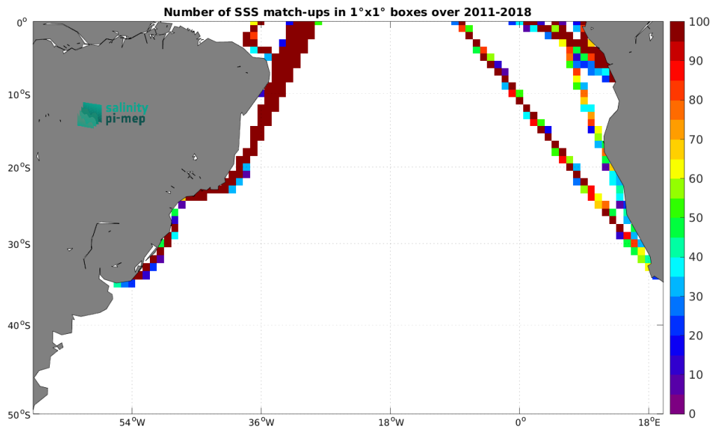
Figure 4: Number of SSS match-ups between TSG (LEGOS-DM) SSS and the SMOS and SMAP SSS L4 OI v1 - 7 Days (LOPS) SSS product for the South Atlantic Ocean Pi-MEP region over 1^\circ \times 1^\circ boxes and for the full satellite product period.
