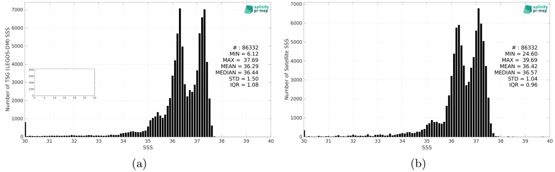
Figure 2: Histograms of SSS from TSG (LEGOS-DM) (a) and SMOS and SMAP SSS L4 OI v1 - 7 Days (LOPS) (b) considering all match-up pairs per bins of 0.1 over the South Atlantic Ocean Pi-MEP region and for the full satellite product period.
