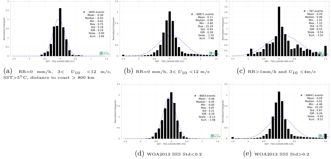
Figure 13: Normalized histogram of \Delta\text{SSS} (SMOS and SMAP SSS L4 OI v1 - 7 Days (LOPS) - TSG (LEGOS-DM)) for 5 different subdatasets corresponding to: RR=0 mm/h, 3 < U_{10} < 12 m/s, SST>5°C, distance to coast > 800 km (a), RR=0 mm/h, 3 < U_{10} < 12 m/s (b), RR>1mm/h and U_{10} < 4 m/s (c), WOA2013 SSS Std<0.2 (d), WOA2013 SSS Std>0.2 (e).
