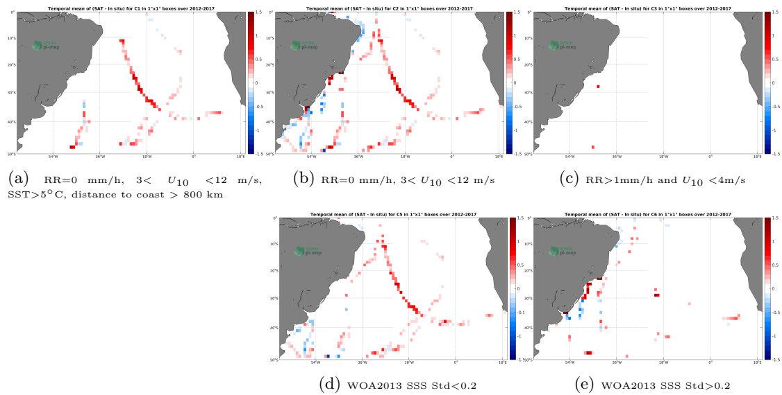
Figure 12: Temporal mean gridded over spatial boxes of size 1^\circ \times 1^\circ of \Delta SSS (SMOS and SMAP SSS L4 OI v1 - 7 Days (LOPS) - TSG (GOSUD-Sailing-ship)) for 5 different subdatasets corresponding to:RR=0 mm/h, 3 < U_{10} < 12 m/s, SST>5°C, distance to coast > 800 km (a), RR=0 mm/h, 3 < U_{10} < 12 m/s (b), RR>1mm/h and U_{10} < 4 m/s (c), WOA2013 SSS Std<0.2 (d), WOA2013 SSS Std>0.2 (e).
