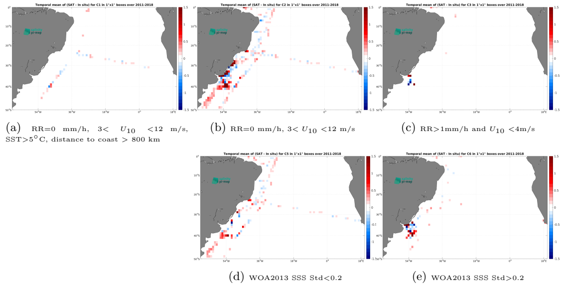
Figure 12: Temporal mean gridded over spatial boxes of size 1^\circ \times 1^\circ of \Delta SSS (SMOS and SMAP SSS L4 OI v1 - 7 Days (LOPS) - TSG (CSIC-UTM)) for 5 different subdatasets corresponding to:RR=0 mm/h, 3 < U_{10} < 12 m/s, SST >5^\circ\text{C} , distance to coast > 800 km (a), RR=0 mm/h, 3 < U_{10} < 12 m/s (b), RR >1 mm/h and U_{10} < 4 m/s (c), WOA2013 SSS Std <0.2 (d), WOA2013 SSS Std >0.2 (e).
