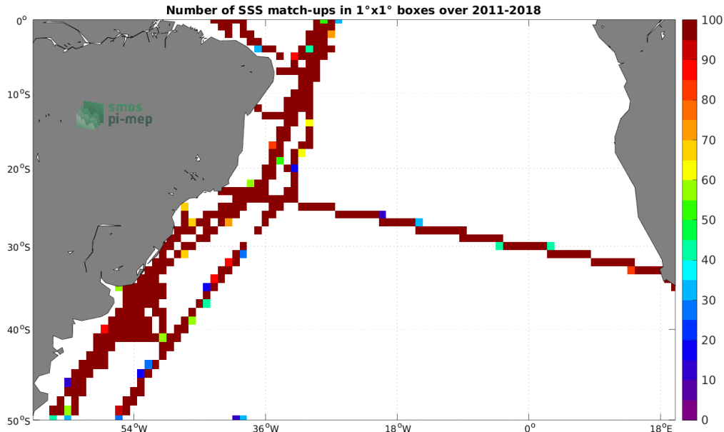
Figure 4: Number of SSS match-ups between TSG (CSIC-UTM) SSS and the SMOS and SMAP SSS L4 OI v1 - 7 Days (LOPS) SSS product for the South Atlantic Ocean Pi-MEP region over 1^\circ \times 1^\circ boxes and for the full satellite product period.
