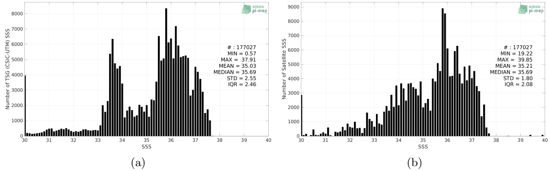
Figure 2: Histograms of SSS from TSG (CSIC-UTM) (a) and SMOS and SMAP SSS L4 OI v1 - 7 Days (LOPS) (b) considering all match-up pairs per bins of 0.1 over the South Atlantic Ocean Pi-MEP region and for the full satellite product period.
