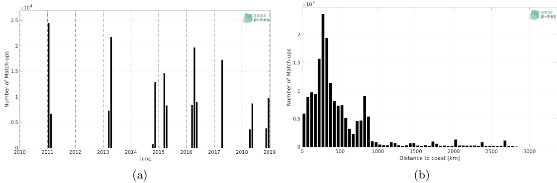
Figure 1: Number of match-ups between TSG (CSIC-UTM) and SMOS and SMAP SSS L4 OI v1 - 7 Days (LOPS) SSS as a function of time (a) and as function of the distance to coast (b) over the South Atlantic Ocean Pi-MEP region and for the full satellite product period.
