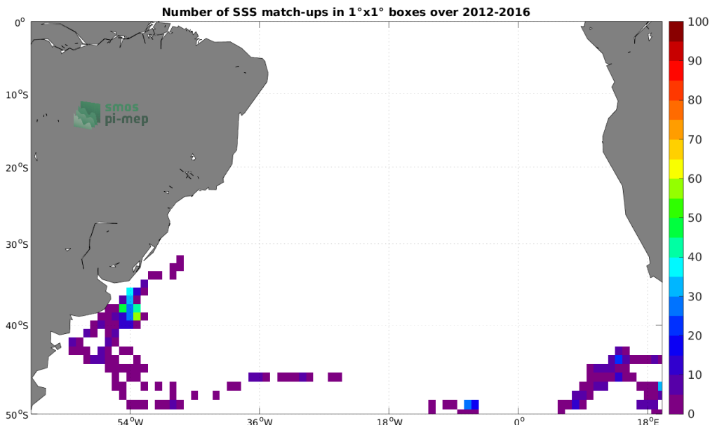
Figure 4: Number of SSS match-ups between Marine mammals SSS and the SMOS and SMAP SSS L4 OI v1 - 7 Days (LOPS) SSS product for the South Atlantic Ocean Pi-MEP region over 1^\circ \times 1^\circ boxes and for the full satellite product period.
