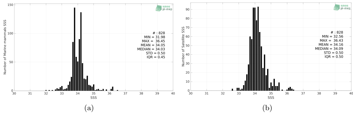
Figure 2: Histograms of SSS from Marine mammals (a) and SMOS and SMAP SSS L4 OI v1 - 7 Days (LOPS) (b) considering all match-up pairs per bins of 0.1 over the South Atlantic Ocean Pi-MEP region and for the full satellite product period.
