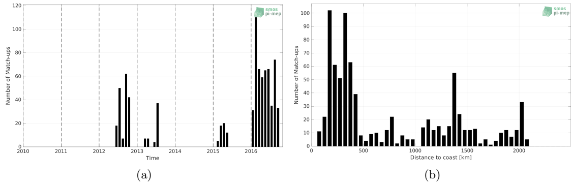
Figure 1: Number of match-ups between Marine mammals and SMOS and SMAP SSS L4 OI v1 - 7 Days (LOPS) SSS as a function of time (a) and as function of the distance to coast (b) over the South Atlantic Ocean Pi-MEP region and for the full satellite product period.
