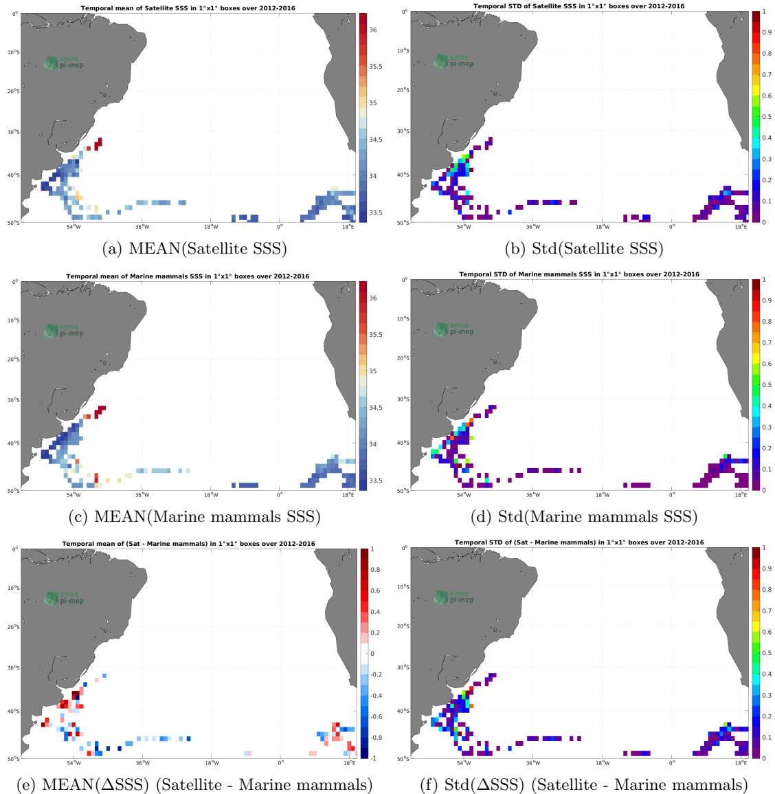
Figure 6: Temporal mean (left) and Std (right) of SSS from SMOS and SMAP SSS L4 OI v1 - 7 Days (LOPS) (top), Marine mammals (middle), and of \Delta SSS (Satellite - Marine mammals). Only match-up pairs are used to generate these maps.
