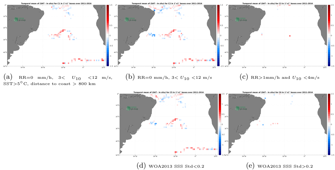
Figure 11: Temporal mean gridded over spatial boxes of size 1^\circ \times 1^\circ of \Delta\text{SSS} (SMOS and SMAP SSS L4 OI v1 - 7 Days (LOPS) - Surface drifters) for 5 different subdatasets corresponding to:RR=0 mm/h, 3 < U_{10} < 12 m/s, SST >5^\circ\text{C} , distance to coast > 800 km (a), RR=0 mm/h, 3 < U_{10} < 12 m/s (b), RR >1 mm/h and U_{10} < 4 m/s (c), WOA2013 SSS Std <0.2 (d), WOA2013 SSS Std >0.2 (e).
