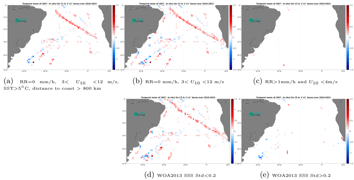
Figure 12: Temporal mean gridded over spatial boxes of size 1^\circ \times 1^\circ of \Delta\text{SSS} (SMOS SSS L4 v1 - Weekly (CMEMS-CNR) - TSG (SAMOS)) for 5 different subdatasets corresponding to:RR=0 mm/h, 3 < U_{10} < 12 m/s, SST >5^\circ\text{C} , distance to coast > 800 km (a), RR=0 mm/h, 3 < U_{10} < 12 m/s (b), RR >1 mm/h and U_{10} < 4 m/s (c), WOA2013 SSS Std <0.2 (d), WOA2013 SSS Std >0.2 (e).
