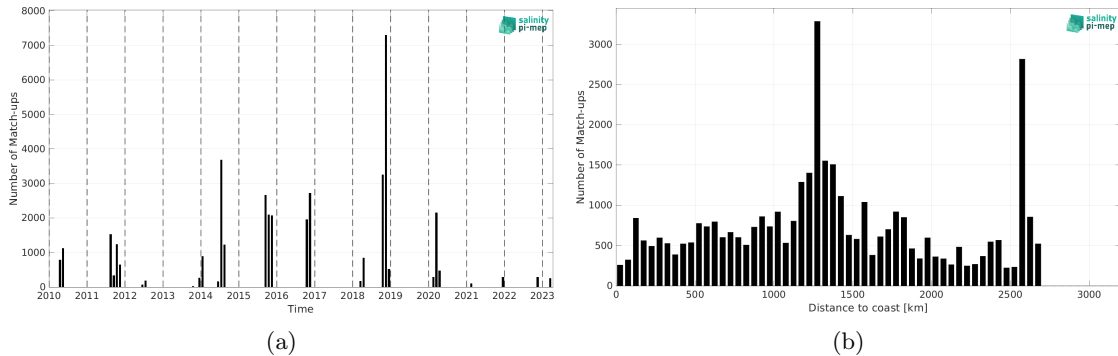
Figure 1: Number of match-ups between TSG (SAMOS) and SMOS SSS L4 v1 - Weekly (CMEMS-CNR) SSS as a function of time (a) and as function of the distance to coast (b) over the South Atlantic Ocean Pi-MEP region and for the full satellite product period.
