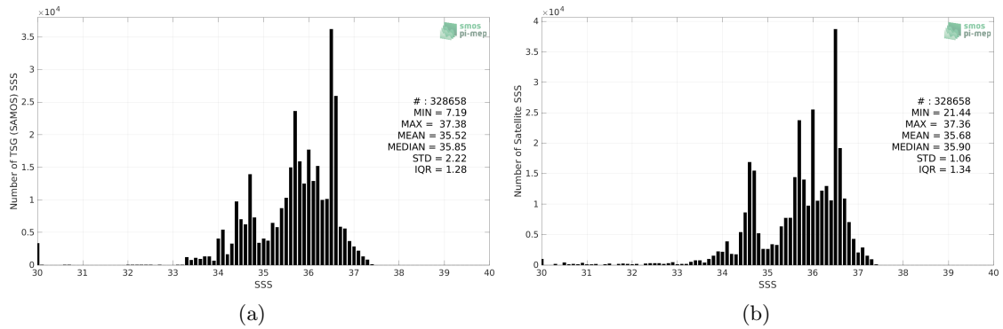
Figure 2: Histograms of SSS from TSG (SAMOS) (a) and SMOS SSS L4 v1 - Weekly (CMEMS-CNR) (b) considering all match-up pairs per bins of 0.1 over the South Atlantic Ocean Pi-MEP region and for the full satellite product period.
