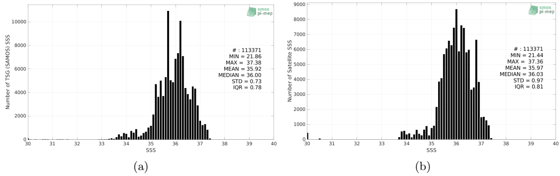
Figure 2: Histograms of SSS from TSG (SAMOS) (a) and SMOS SSS L4 v1 - Weekly (CMEMS-CNR) (b) considering all match-up pairs per bins of 0.1 over the South Atlantic Ocean Pi-MEP region and for the full satellite product period.
