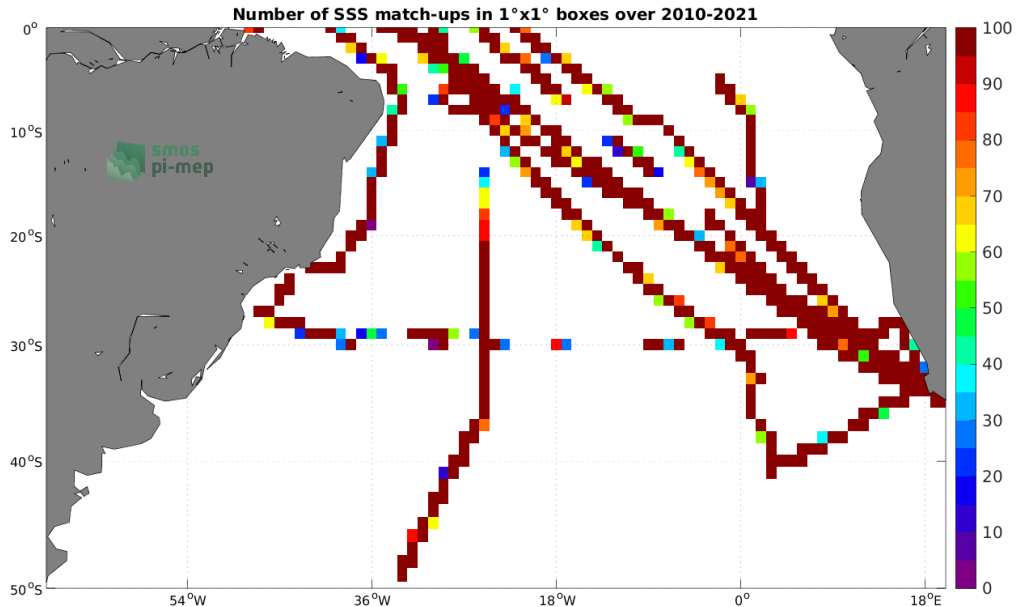
Figure 4: Number of SSS match-ups between TSG (SAMOS) SSS and the SMOS SSS L4 v1 - Weekly (CMEMS-CNR) SSS product for the South Atlantic Ocean Pi-MEP region over 1^\circ \times 1^\circ boxes and for the full satellite product period.
