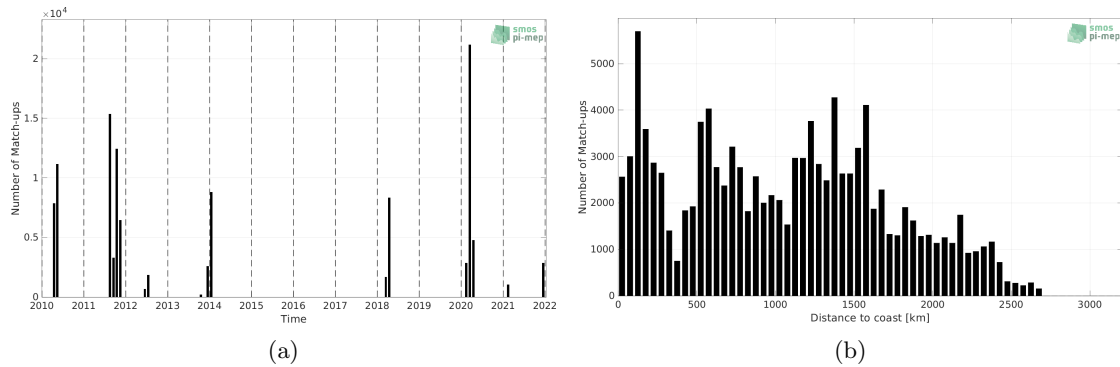
Figure 1: Number of match-ups between TSG (SAMOS) and SMOS SSS L4 v1 - Weekly (CMEMS-CNR) SSS as a function of time (a) and as function of the distance to coast (b) over the South Atlantic Ocean Pi-MEP region and for the full satellite product period.
