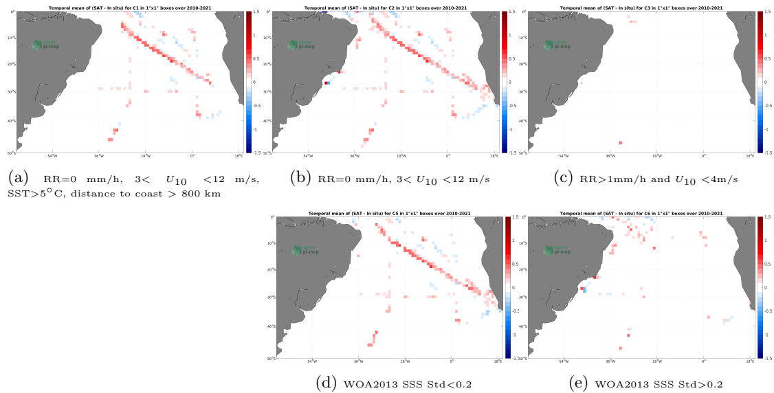
Figure 12: Temporal mean gridded over spatial boxes of size 1^\circ \times 1^\circ of \Delta\text{SSS} (SMOS SSS L4 v1 - Weekly (CMEMS-CNR) - TSG (SAMOS)) for 5 different subdatasets corresponding to:RR=0 mm/h, 3 < U_{10} < 12 m/s, SST >5^\circ\text{C} , distance to coast > 800 km (a), RR=0 mm/h, 3 < U_{10} < 12 m/s (b), RR >1 mm/h and U_{10} < 4 m/s (c), WOA2013 SSS Std <0.2 (d), WOA2013 SSS Std >0.2 (e).
