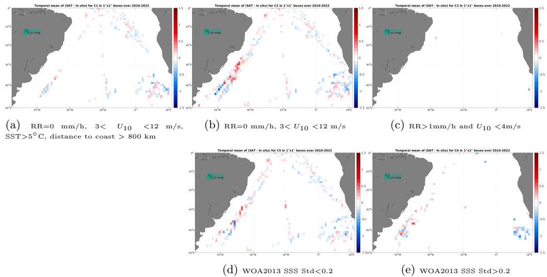
Figure 12: Temporal mean gridded over spatial boxes of size 1^\circ \times 1^\circ of \Delta\text{SSS} (SMOS SSS L4 v1 - Weekly (CMEMS-CNR) - TSG (Polarstern)) for 5 different subdatasets corresponding to:RR=0 mm/h, 3 < U_{10} < 12 m/s, SST >5^\circ\text{C} , distance to coast > 800 km (a), RR=0 mm/h, 3 < U_{10} < 12 m/s (b), RR >1 mm/h and U_{10} < 4 m/s (c), WOA2013 SSS Std <0.2 (d), WOA2013 SSS Std >0.2 (e).
