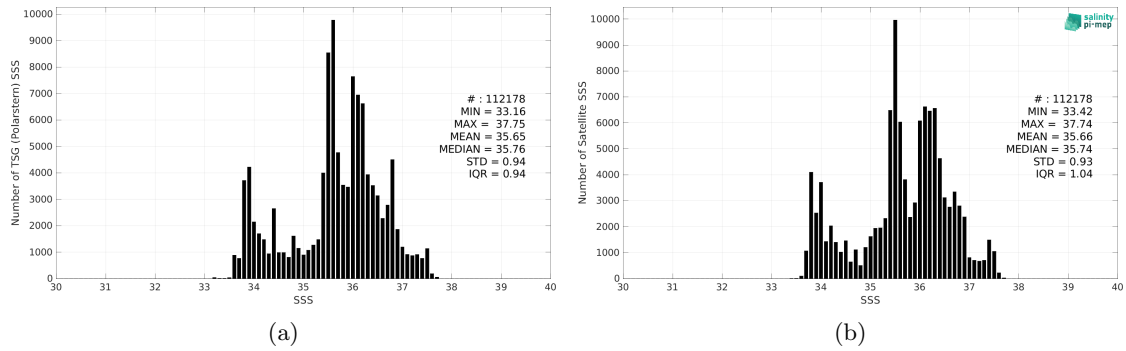
Figure 2: Histograms of SSS from TSG (Polarstern) (a) and SMOS SSS L4 v1 - Weekly (CMEMS-CNR) (b) considering all match-up pairs per bins of 0.1 over the South Atlantic Ocean Pi-MEP region and for the full satellite product period.
