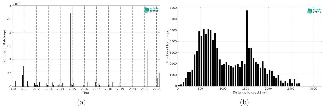
Figure 1: Number of match-ups between TSG (Polarstern) and SMOS SSS L4 v1 - Weekly (CMEMS-CNR) SSS as a function of time (a) and as function of the distance to coast (b) over the South Atlantic Ocean Pi-MEP region and for the full satellite product period.
