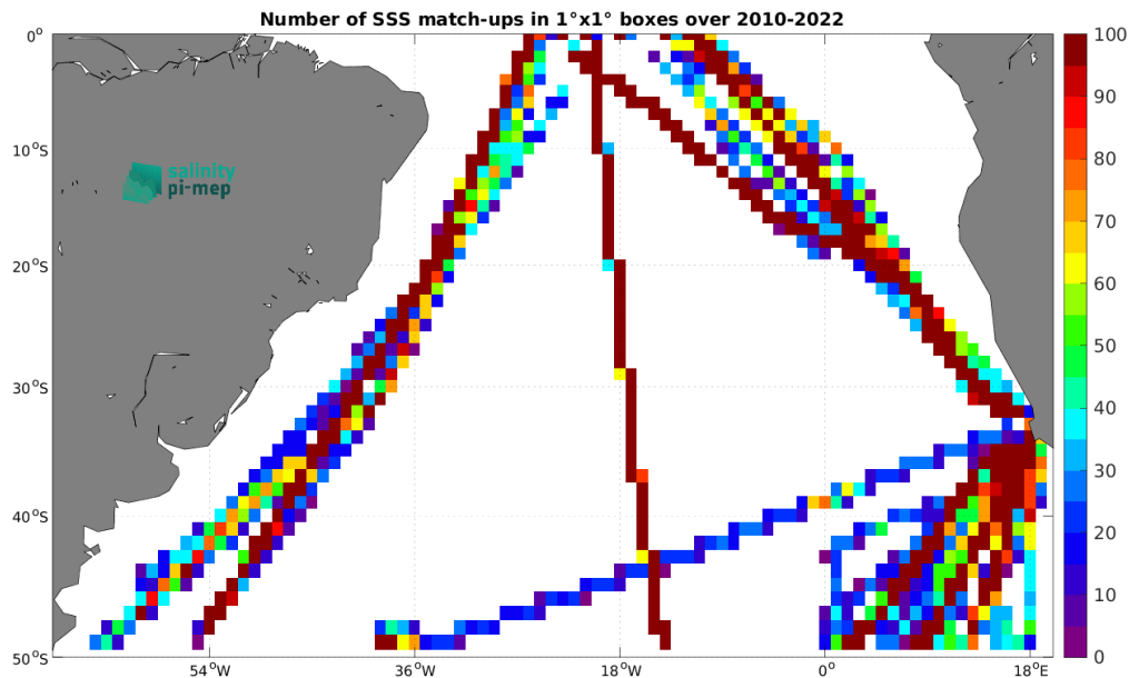
Figure 4: Number of SSS match-ups between TSG (Polarstern) SSS and the SMOS SSS L4 v1 - Weekly (CMEMS-CNR) SSS product for the South Atlantic Ocean Pi-MEP region over 1^\circ \times 1^\circ boxes and for the full satellite product period.
