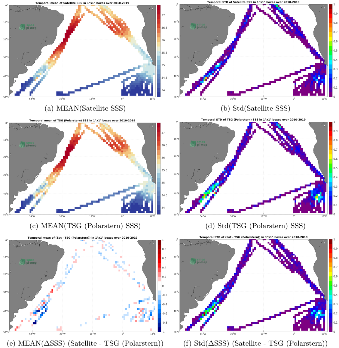
Figure 6: Temporal mean (left) and Std (right) of SSS from SMOS SSS L4 v1 - Weekly (CMEMS-CNR) (top), TSG (Polarstern) (middle), and of \Delta SSS (Satellite - TSG (Polarstern)). Only match-up pairs are used to generate these maps.
