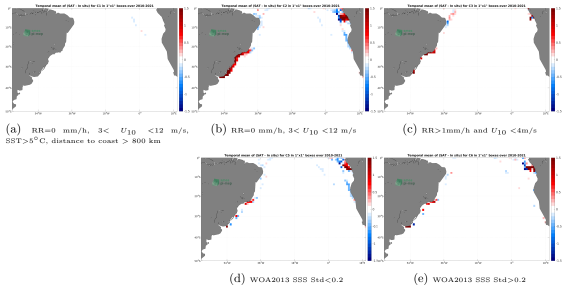
Figure 12: Temporal mean gridded over spatial boxes of size 1^\circ \times 1^\circ of \Delta\text{SSS} (SMOS SSS L4 v1 - Weekly (CMEMS-CNR) - TSG (LEGOS-DM)) for 5 different subdatasets corresponding to:RR=0 mm/h, 3 < U_{10} < 12 m/s, SST >5^\circ\text{C} , distance to coast > 800 km (a), RR=0 mm/h, 3 < U_{10} < 12 m/s (b), RR >1 mm/h and U_{10} < 4 m/s (c), WOA2013 SSS Std <0.2 (d), WOA2013 SSS Std >0.2 (e).
