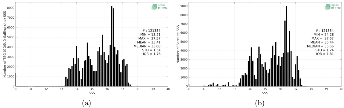
Figure 2: Histograms of SSS from TSG (GOSUD-Sailing-ship) (a) and SMOS SSS L4 v1 - Weekly (CMEMS-CNR) (b) considering all match-up pairs per bins of 0.1 over the South Atlantic Ocean Pi-MEP region and for the full satellite product period.
