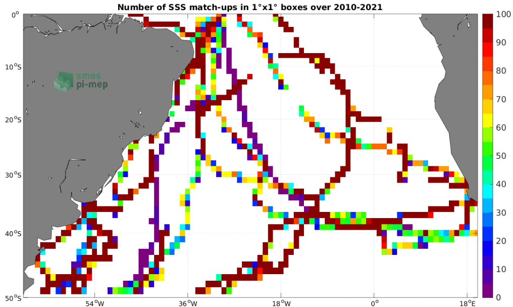
Figure 4: Number of SSS match-ups between TSG (GOSUD-Sailing-ship) SSS and the SMOS SSS L4 v1 - Weekly (CMEMS-CNR) SSS product for the South Atlantic Ocean Pi-MEP region over 1^\circ \times 1^\circ boxes and for the full satellite product period.
