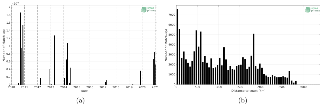
Figure 1: Number of match-ups between TSG (GOSUD-Sailing-ship) and SMOS SSS L4 v1 - Weekly (CMEMS-CNR) SSS as a function of time (a) and as function of the distance to coast (b) over the South Atlantic Ocean Pi-MEP region and for the full satellite product period.
