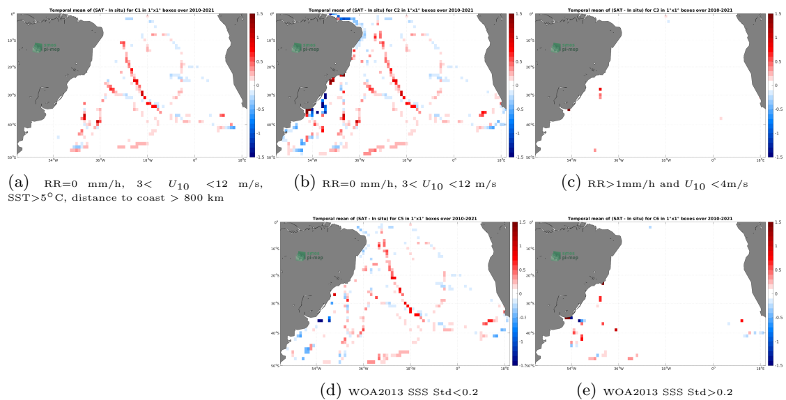
Figure 12: Temporal mean gridded over spatial boxes of size 1^\circ \times 1^\circ of \Delta\text{SSS} (SMOS SSS L4 v1 - Weekly (CMEMS-CNR) - TSG (GOSUD-Sailing-ship)) for 5 different subdatasets corresponding to:RR=0 mm/h, 3 < U_{10} < 12 m/s, SST >5^\circ\text{C} , distance to coast > 800 km (a), RR=0 mm/h, 3 < U_{10} < 12 m/s (b), RR >1 mm/h and U_{10} < 4 m/s (c), WOA2013 SSS Std <0.2 (d), WOA2013 SSS Std >0.2 (e).
