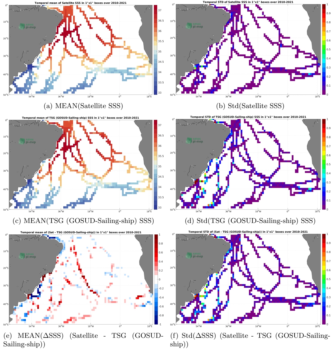
Figure 6: Temporal mean (left) and Std (right) of SSS from SMOS SSS L4 v1 - Weekly (CMEMS-CNR) (top), TSG (GOSUD-Sailing-ship) (middle), and of \Delta SSS (Satellite - TSG (GOSUD-Sailing-ship)). Only match-up pairs are used to generate these maps.
