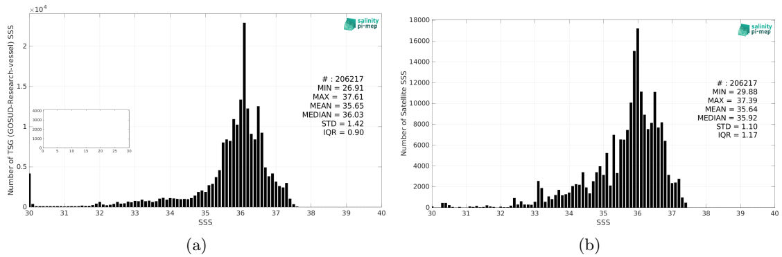
Figure 2: Histograms of SSS from TSG (GOSUD-Research-vessel) (a) and SMOS SSS L4 v1 - Weekly (CMEMS-CNR) (b) considering all match-up pairs per bins of 0.1 over the South Atlantic Ocean Pi-MEP region and for the full satellite product period.
