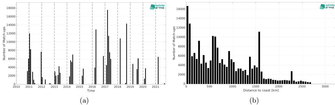
Figure 1: Number of match-ups between TSG (GOSUD-Research-vessel) and SMOS SSS L4 v1 - Weekly (CMEMS-CNR) SSS as a function of time (a) and as function of the distance to coast (b) over the South Atlantic Ocean Pi-MEP region and for the full satellite product period.
