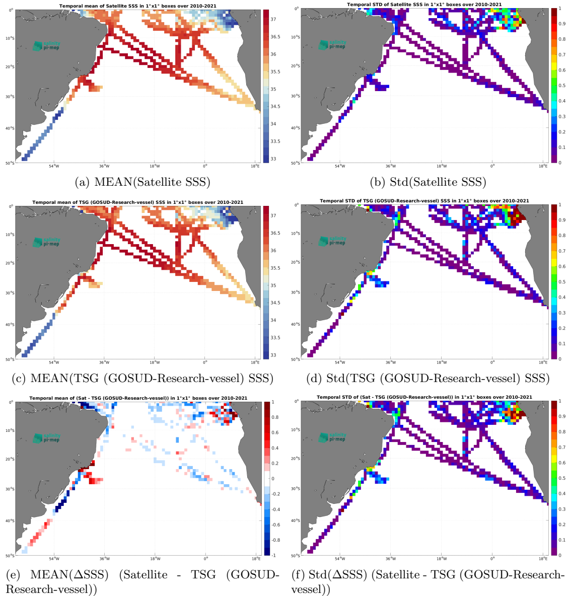
Figure 6: Temporal mean (left) and Std (right) of SSS from SMOS SSS L4 v1 - Weekly (CMEMS-CNR) (top), TSG (GOSUD-Research-vessel) (middle), and of \Delta SSS (Satellite - TSG (GOSUD-Research-vessel)). Only match-up pairs are used to generate these maps.
