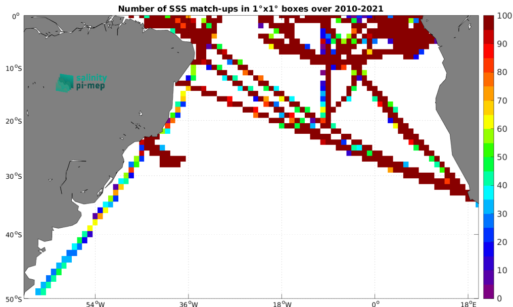
Figure 4: Number of SSS match-ups between TSG (GOSUD-Research-vessel) SSS and the SMOS SSS L4 v1 - Weekly (CMEMS-CNR) SSS product for the South Atlantic Ocean Pi-MEP region over 1^\circ \times 1^\circ boxes and for the full satellite product period.
