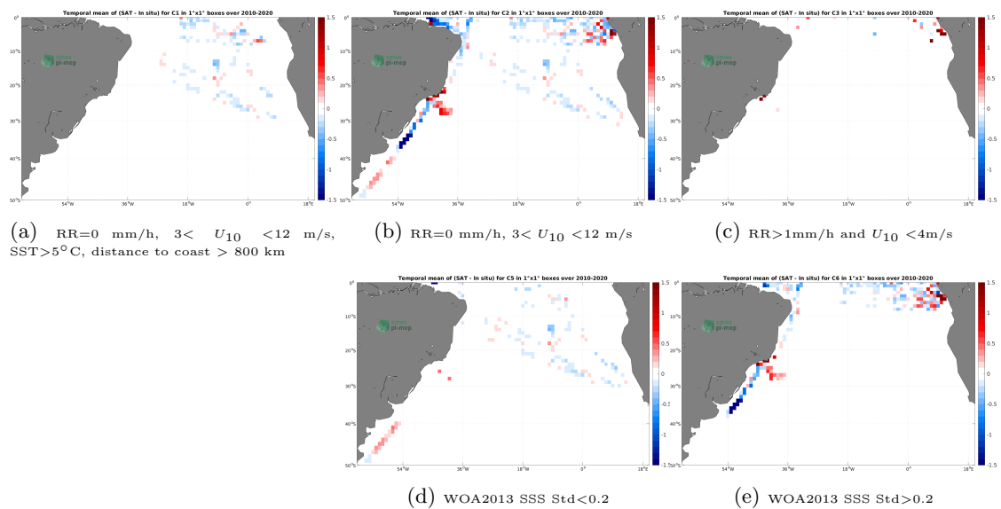
Figure 12: Temporal mean gridded over spatial boxes of size 1^\circ \times 1^\circ of \Delta SSS (SMOS SSS L4 v1 - Weekly (CMEMS-CNR) - TSG (GOSUD-Research-vessel)) for 5 different subdatasets corresponding to:RR=0 mm/h, 3 < U_{10} < 12 m/s, SST >5^\circ\text{C} , distance to coast > 800 km (a), RR=0 mm/h, 3 < U_{10} < 12 m/s (b), RR >1 mm/h and U_{10} < 4 m/s (c), WOA2013 SSS Std <0.2 (d), WOA2013 SSS Std >0.2 (e).
