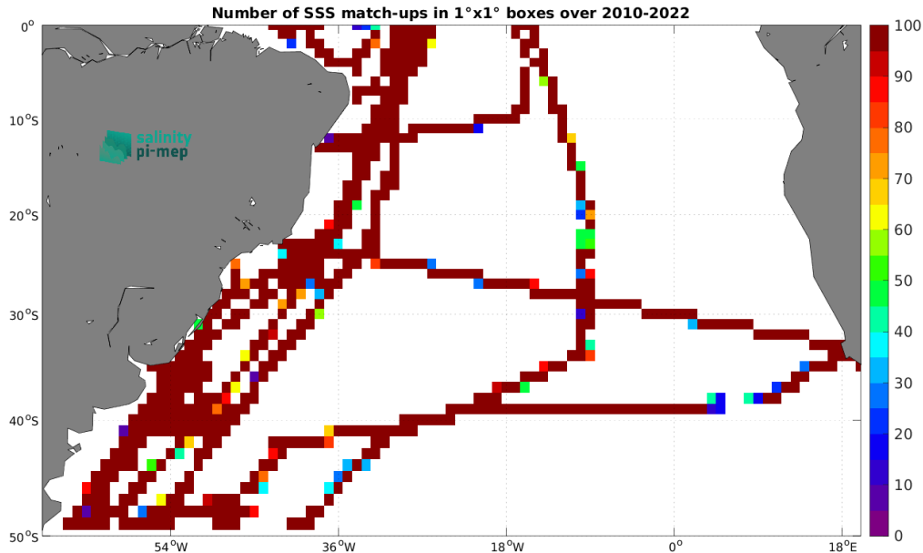
Figure 4: Number of SSS match-ups between TSG (CSIC-UTM) SSS and the SMOS SSS L4 v1 - Weekly (CMEMS-CNR) SSS product for the South Atlantic Ocean Pi-MEP region over 1^\circ \times 1^\circ boxes and for the full satellite product period.
