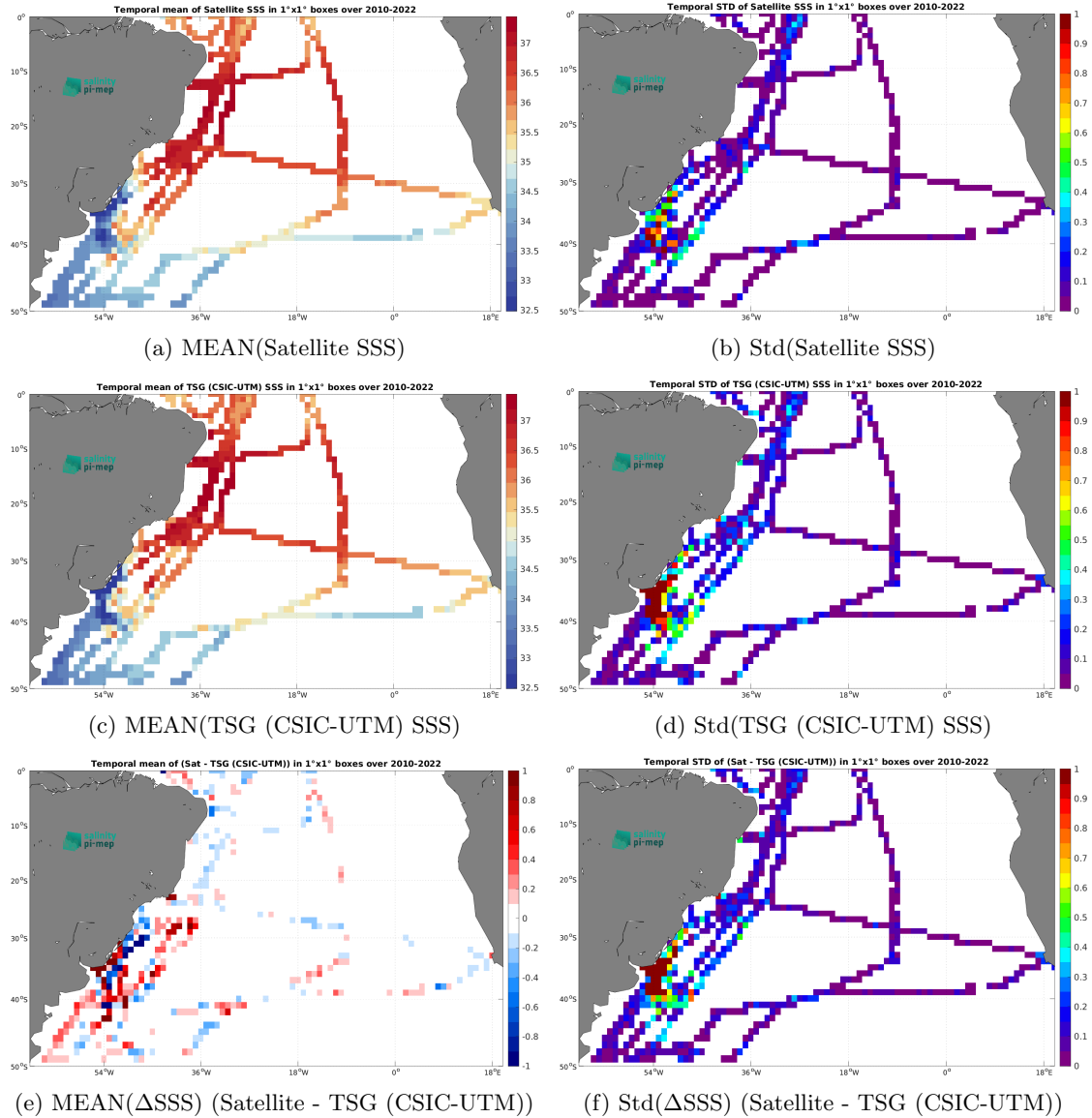
Figure 6: Temporal mean (left) and Std (right) of SSS from SMOS SSS L4 v1 - Weekly (CMEMS-CNR) (top), TSG (CSIC-UTM) (middle), and of \Delta SSS (Satellite - TSG (CSIC-UTM)). Only match-up pairs are used to generate these maps.
