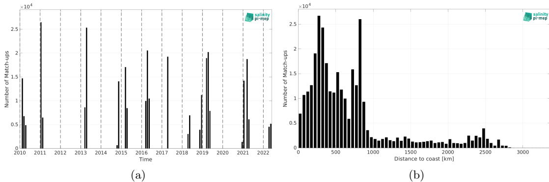
Figure 1: Number of match-ups between TSG (CSIC-UTM) and SMOS SSS L4 v1 - Weekly (CMEMS-CNR) SSS as a function of time (a) and as function of the distance to coast (b) over the South Atlantic Ocean Pi-MEP region and for the full satellite product period.
