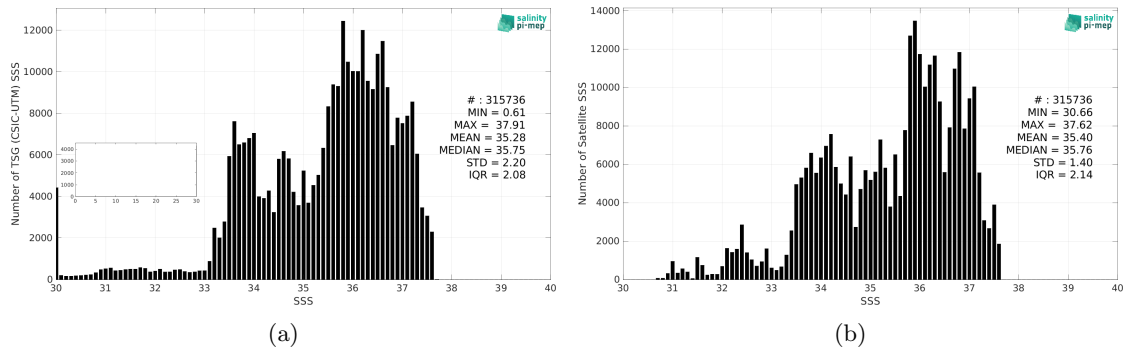
Figure 2: Histograms of SSS from TSG (CSIC-UTM) (a) and SMOS SSS L4 v1 - Weekly (CMEMS-CNR) (b) considering all match-up pairs per bins of 0.1 over the South Atlantic Ocean Pi-MEP region and for the full satellite product period.
