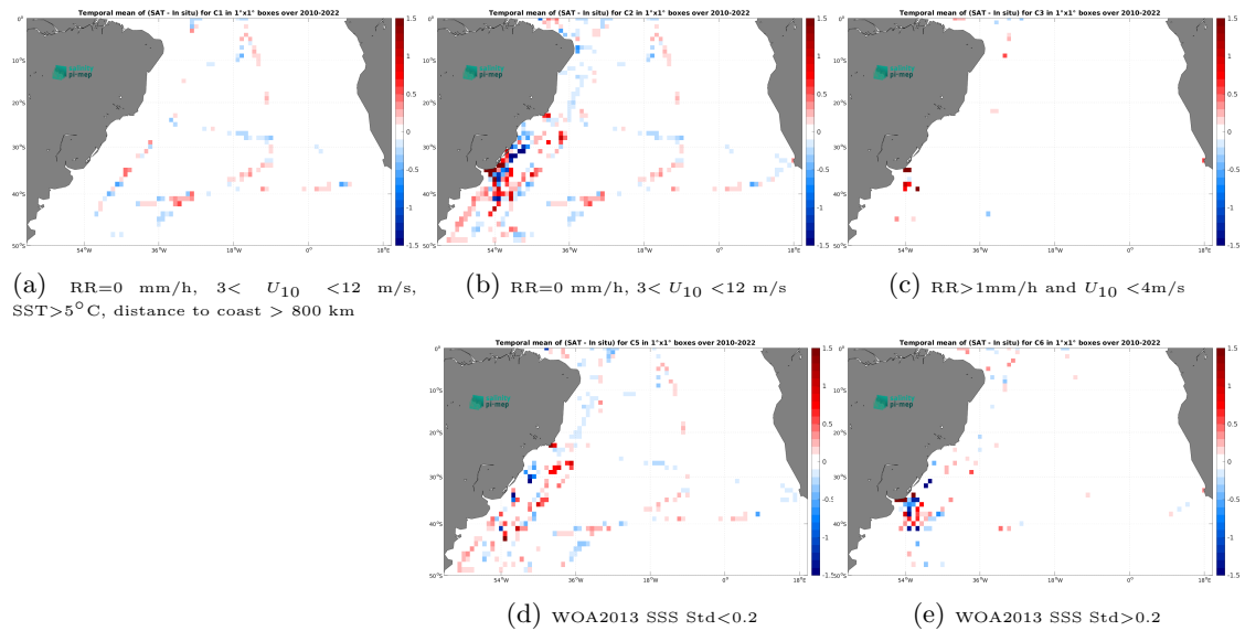
Figure 12: Temporal mean gridded over spatial boxes of size 1^\circ \times 1^\circ of \Delta\text{SSS} (SMOS SSS L4 v1 - Weekly (CMEMS-CNR) - TSG (CSIC-UTM)) for 5 different subdatasets corresponding to:RR=0 mm/h, 3 < U_{10} < 12 m/s, SST >5^\circ\text{C} , distance to coast > 800 km (a), RR=0 mm/h, 3 < U_{10} < 12 m/s (b), RR >1 mm/h and U_{10} < 4 m/s (c), WOA2013 SSS Std <0.2 (d), WOA2013 SSS Std >0.2 (e).
