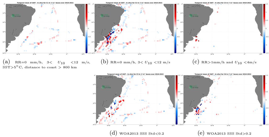
Figure 12: Temporal mean gridded over spatial boxes of size 1^\circ \times 1^\circ of \Delta\text{SSS} (SMOS SSS L4 v1 - Weekly (CMEMS-CNR) - TSG (CSIC-UTM)) for 5 different subdatasets corresponding to:RR=0 mm/h, 3 < U_{10} < 12 m/s, SST >5^\circ\text{C} , distance to coast > 800 km (a), RR=0 mm/h, 3 < U_{10} < 12 m/s (b), RR >1 mm/h and U_{10} < 4 m/s (c), WOA2013 SSS Std <0.2 (d), WOA2013 SSS Std >0.2 (e).
