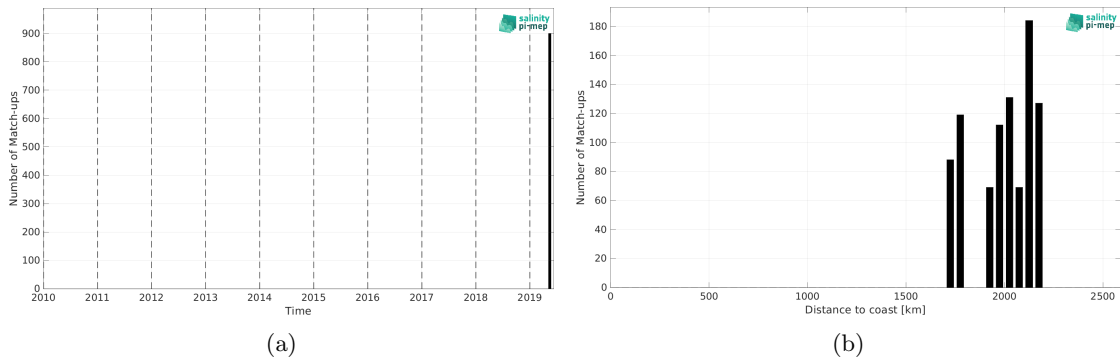
Figure 1: Number of match-ups between Saildrone and SMOS SSS L4 v1 - Weekly (CMEMS-CNR) SSS as a function of time (a) and as function of the distance to coast (b) over the South Atlantic Ocean Pi-MEP region and for the full satellite product period.
