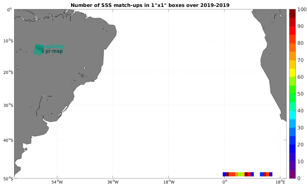
Figure 4: Number of SSS match-ups between Saldrone SSS and the SMOS SSS L4 v1 - Weekly (CMEMS-CNR) SSS product for the South Atlantic Ocean Pi-MEP region over 1^\circ \times 1^\circ boxes and for the full satellite product period.
