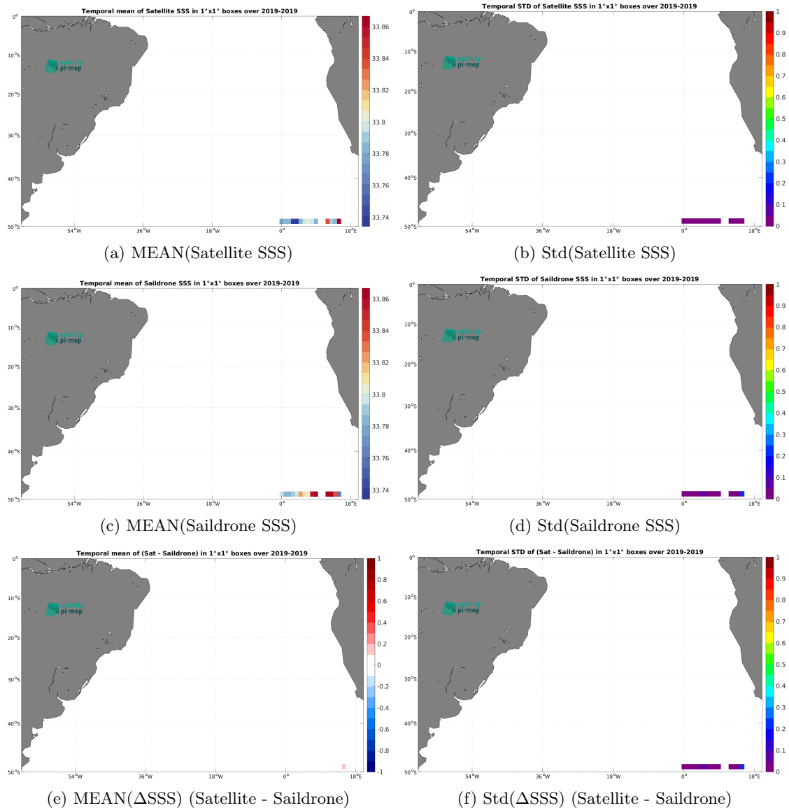
Figure 6: Temporal mean (left) and Std (right) of SSS from SMOS SSS L4 v1 - Weekly (CMEMS-CNR) (top), Saildrone (middle), and of \Delta SSS (Satellite - Saildrone). Only match-up pairs are used to generate these maps.
