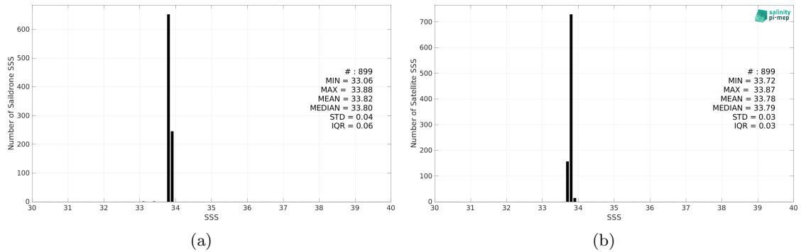
Figure 2: Histograms of SSS from Saildrone (a) and SMOS SSS L4 v1 - Weekly (CMEMS-CNR) (b) considering all match-up pairs per bins of 0.1 over the South Atlantic Ocean Pi-MEP region and for the full satellite product period.
