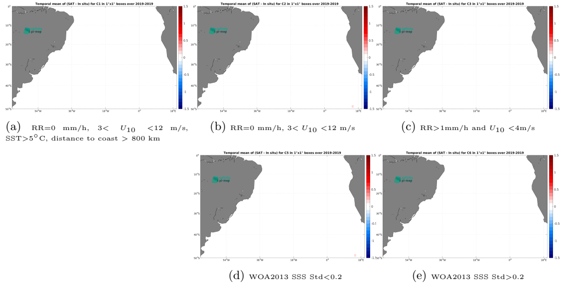
Figure 12: Temporal mean gridded over spatial boxes of size 1^{\circ}\times 1^{\circ} of \Delta\text{SSS} (SMOS SSS L4 v1 - Weekly (CMEMS-CNR) - Saildrone) for 5 different subdatasets corresponding to:RR=0 mm/h, 3 < U_{10} < 12 m/s, SST >5^{\circ}\text{C} , distance to coast > 800 km (a), RR=0 mm/h, 3 < U_{10} < 12 m/s (b), RR >1 mm/h and U_{10} < 4 m/s (c), WOA2013 SSS Std <0.2 (d), WOA2013 SSS Std >0.2 (e).
