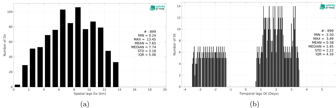
Figure 5: Histograms of the spatial (a) and temporal (b) lags between the location/time of the Saldrone measurement and the date of the corresponding SMOS SSS L4 v1 - Weekly (CMEMS-CNR) SSS pixel.
