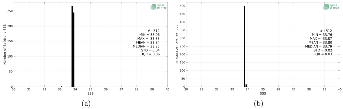
Figure 2: Histograms of SSS from Sairdrone (a) and SMOS SSS L4 v1 - Weekly (CMEMS-CNR) (b) considering all match-up pairs per bins of 0.1 over the South Atlantic Ocean Pi-MEP region and for the full satellite product period.
