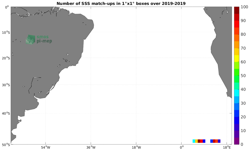
Figure 4: Number of SSS match-ups between Saildrone SSS and the SMOS SSS L4 v1 - Weekly (CMEMS-CNR) SSS product for the South Atlantic Ocean Pi-MEP region over 1^\circ \times 1^\circ boxes and for the full satellite product period.
