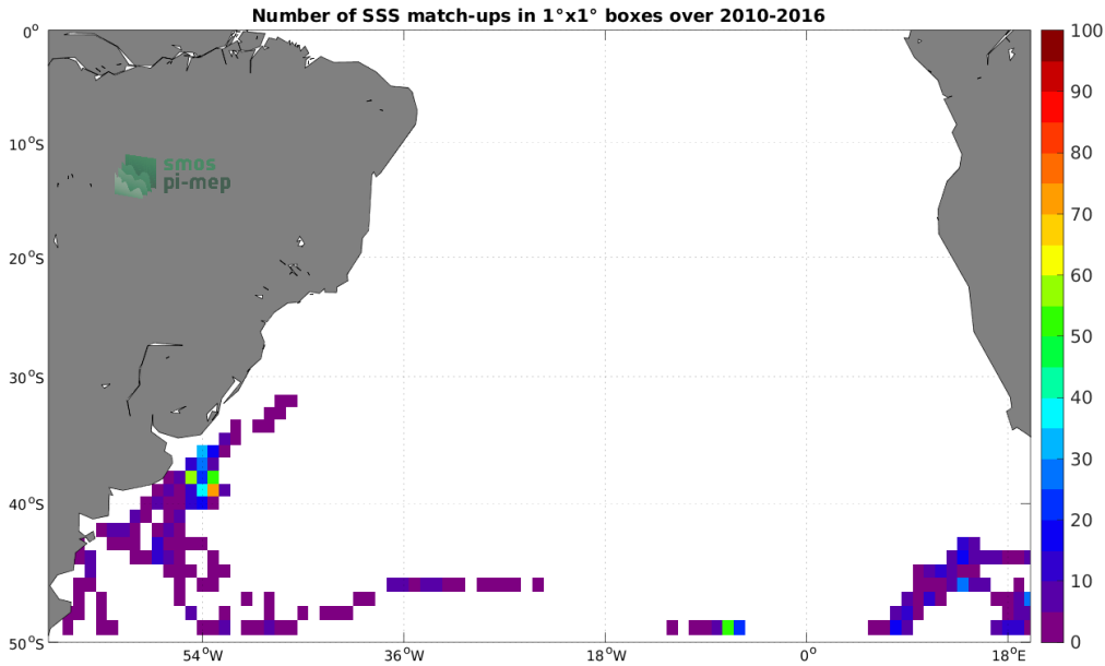
Figure 4: Number of SSS match-ups between Marine mammals SSS and the SMOS SSS L4 v1 - Weekly (CMEMS-CNR) SSS product for the South Atlantic Ocean Pi-MEP region over 1^\circ \times 1^\circ boxes and for the full satellite product period.
