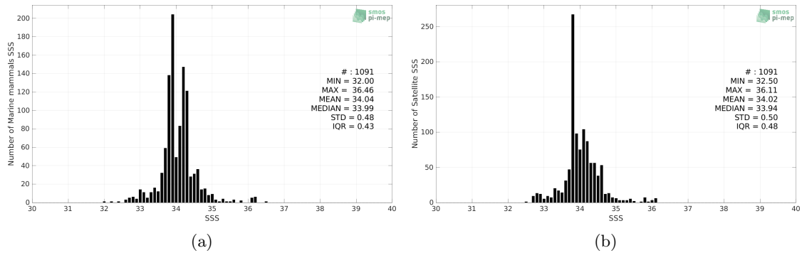
Figure 2: Histograms of SSS from Marine mammals (a) and SMOS SSS L4 v1 - Weekly (CMEMS-CNR) (b) considering all match-up pairs per bins of 0.1 over the South Atlantic Ocean Pi-MEP region and for the full satellite product period.
