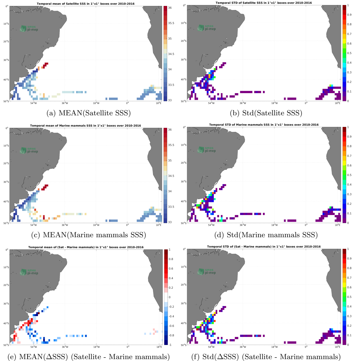
Figure 6: Temporal mean (left) and Std (right) of SSS from SMOS SSS L4 v1 - Weekly (CMEMS-CNR) (top), Marine mammals (middle), and of \Delta SSS (Satellite - Marine mammals). Only match-up pairs are used to generate these maps.
