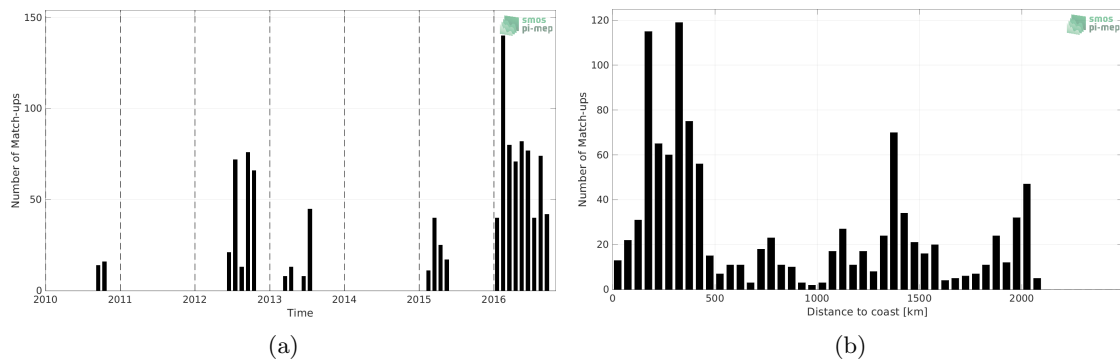
Figure 1: Number of match-ups between Marine mammals and SMOS SSS L4 v1 - Weekly (CMEMS-CNR) SSS as a function of time (a) and as function of the distance to coast (b) over the South Atlantic Ocean Pi-MEP region and for the full satellite product period.
