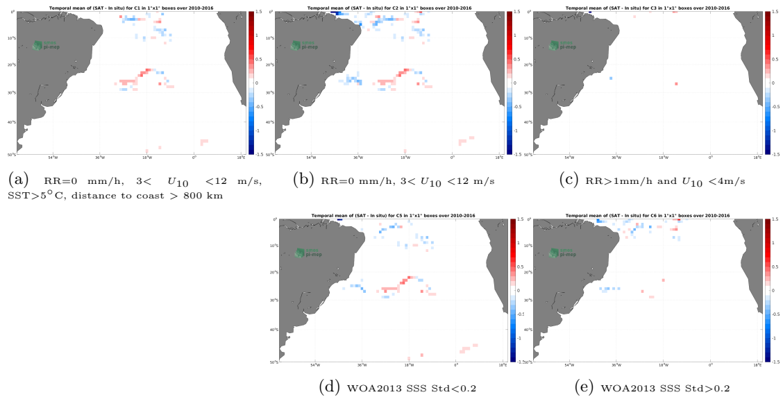
Figure 11: Temporal mean gridded over spatial boxes of size 1^\circ \times 1^\circ of \Delta\text{SSS} (SMOS SSS L4 v1 - Weekly (CMEMS-CNR) - Surface drifters) for 5 different subdatasets corresponding to:RR=0 mm/h, 3 < U_{10} < 12 m/s, SST >5^\circ\text{C} , distance to coast > 800 km (a), RR=0 mm/h, 3 < U_{10} < 12 m/s (b), RR >1 mm/h and U_{10} < 4 m/s (c), WOA2013 SSS Std <0.2 (d), WOA2013 SSS Std >0.2 (e).
