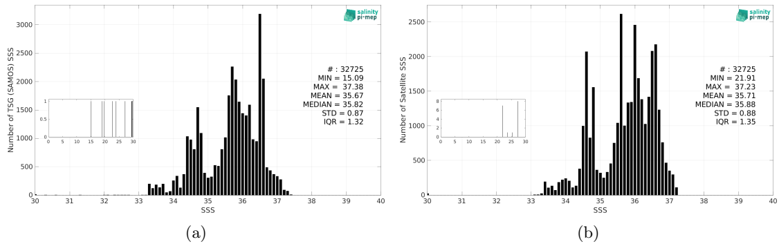
Figure 3: Histograms of SSS from TSG (SAMOS) (a) and SMOS SSS L4 v1 - Monthly (CMEMS-CNR) (b) considering all match-up pairs per bins of 0.1 over the South Atlantic Ocean Pi-MEP region and for the full satellite product period.
