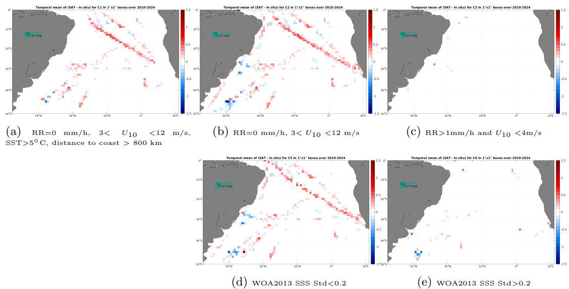
Figure 14: Temporal mean gridded over spatial boxes of size 1^\circ \times 1^\circ of \Delta SSS (SMOS SSS L4 v1 - Monthly (CMEMS-CNR) - TSG (SAMOS)) for 5 different subdatasets corresponding to:RR=0 mm/h, 3 < U_{10} < 12 m/s, SST >5^\circ\text{C} , distance to coast > 800 km (a), RR=0 mm/h, 3 < U_{10} < 12 m/s (b), RR >1 mm/h and U_{10} < 4 m/s (c), WOA2013 SSS Std <0.2 (d), WOA2013 SSS Std >0.2 (e).
