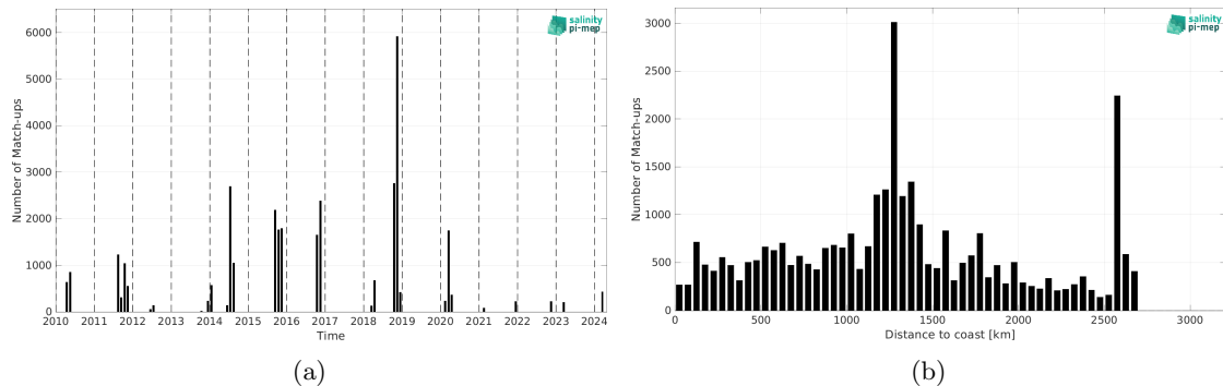
Figure 2: Number of match-ups between TSG (SAMOS) and SMOS SSS L4 v1 - Monthly (CMEMS-CNR) SSS as a function of time (a) and as function of the distance to coast (b) over the South Atlantic Ocean Pi-MEP region and for the full satellite product period.
