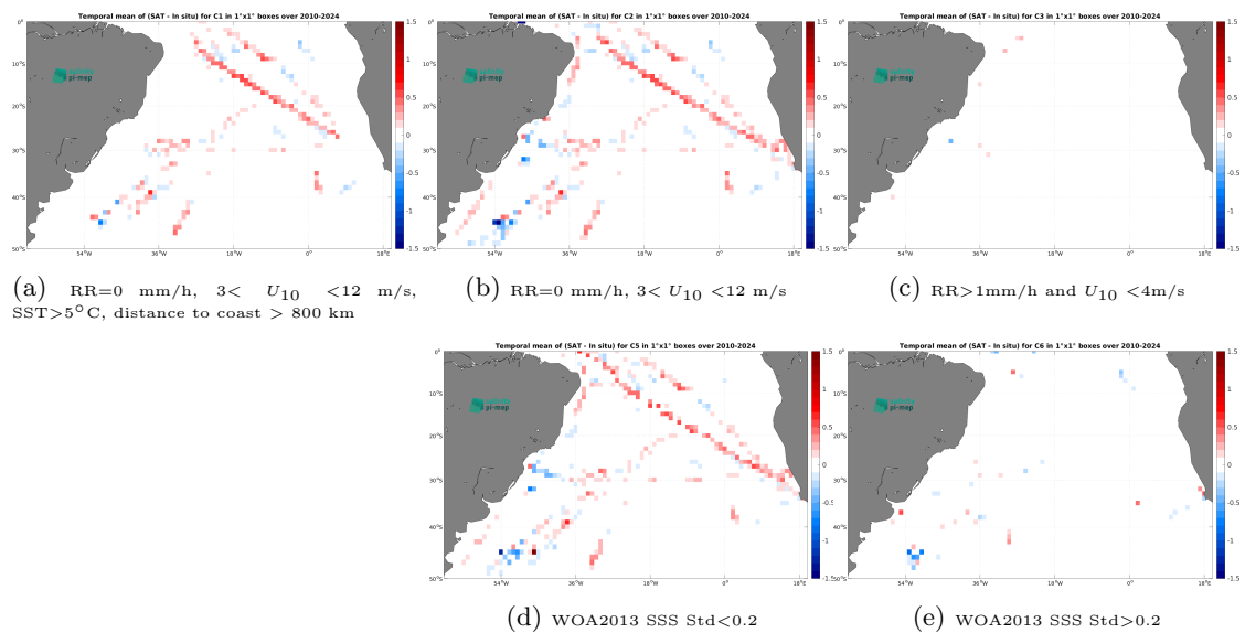
Figure 14: Temporal mean gridded over spatial boxes of size 1^\circ \times 1^\circ of \Delta\text{SSS} (SMOS SSS L4 v1 - Monthly (CMEMS-CNR) - TSG (SAMOS)) for 5 different subdatasets corresponding to:RR=0 mm/h, 3 < U_{10} < 12 m/s, SST >5^\circ\text{C} , distance to coast > 800 km (a), RR=0 mm/h, 3 < U_{10} < 12 m/s (b), RR >1 mm/h and U_{10} < 4 m/s (c), WOA2013 SSS Std <0.2 (d), WOA2013 SSS Std >0.2 (e).
