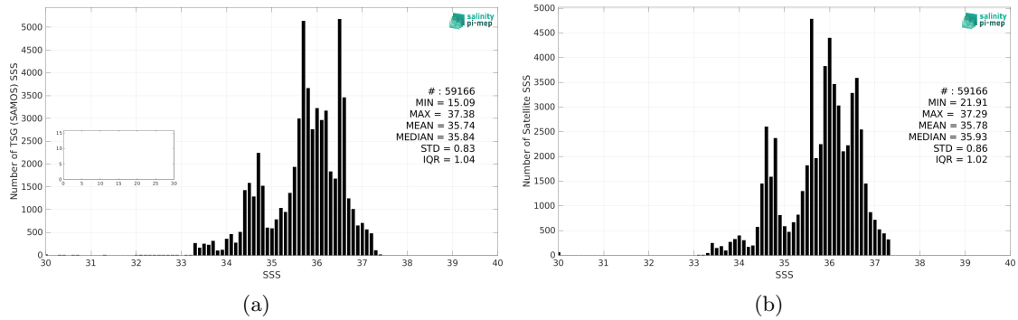
Figure 2: Histograms of SSS from TSG (SAMOS) (a) and SMOS SSS L4 v1 - Monthly (CMEMS-CNR) (b) considering all match-up pairs per bins of 0.1 over the South Atlantic Ocean Pi-MEP region and for the full satellite product period.
