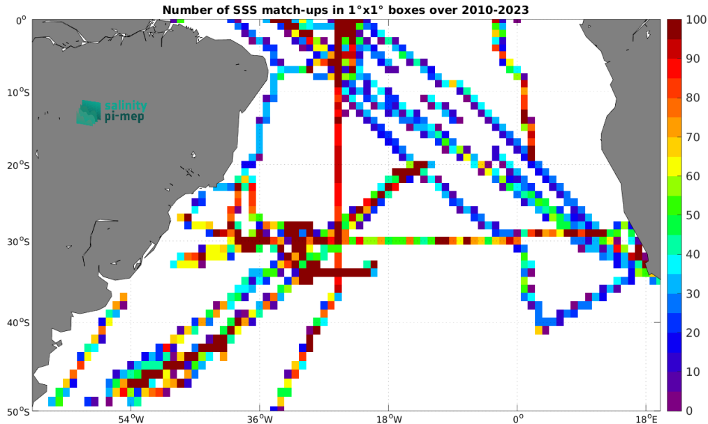
Figure 4: Number of SSS match-ups between TSG (SAMOS) SSS and the SMOS SSS L4 v1 - Monthly (CMEMS-CNR) SSS product for the South Atlantic Ocean Pi-MEP region over 1^\circ \times 1^\circ boxes and for the full satellite product period.
