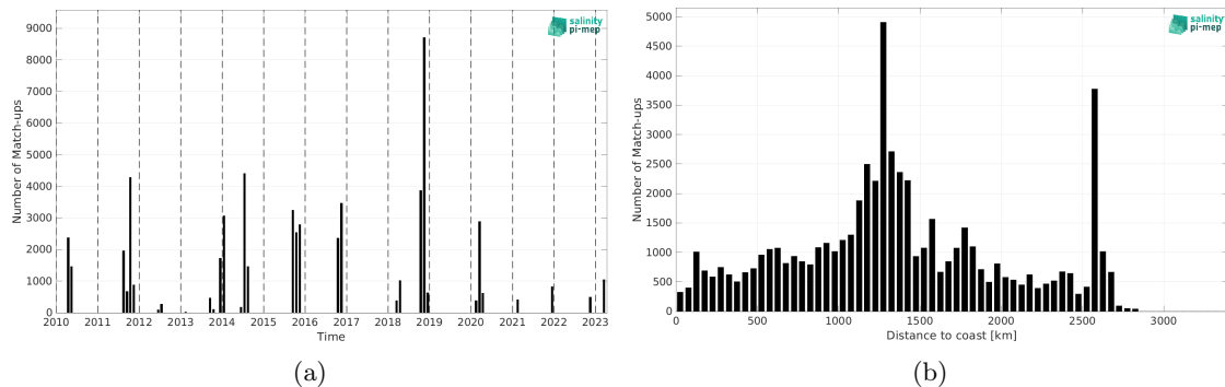
Figure 1: Number of match-ups between TSG (SAMOS) and SMOS SSS L4 v1 - Monthly (CMEMS-CNR) SSS as a function of time (a) and as function of the distance to coast (b) over the South Atlantic Ocean Pi-MEP region and for the full satellite product period.
