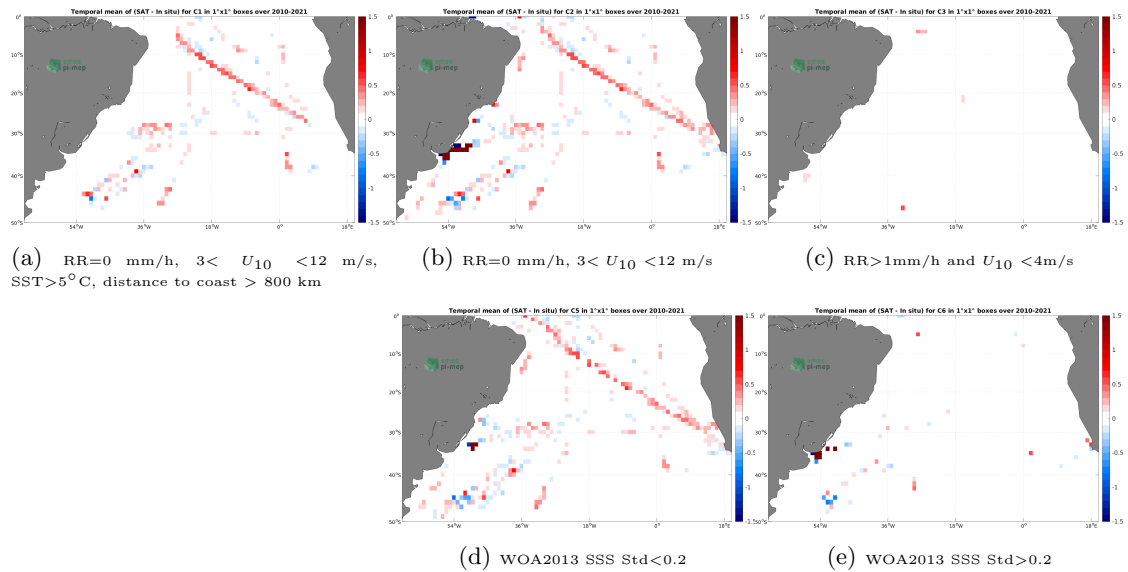
Figure 12: Temporal mean gridded over spatial boxes of size 1^\circ \times 1^\circ of \Delta\text{SSS} (SMOS SSS L4 v1 - Monthly (CMEMS-CNR) - TSG (SAMOS)) for 5 different subdatasets corresponding to:RR=0 mm/h, 3 < U_{10} < 12 m/s, SST >5^\circ\text{C} , distance to coast > 800 km (a), RR=0 mm/h, 3 < U_{10} < 12 m/s (b), RR >1 mm/h and U_{10} < 4 m/s (c), WOA2013 SSS Std <0.2 (d), WOA2013 SSS Std >0.2 (e).
