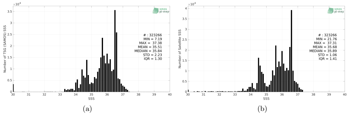
Figure 2: Histograms of SSS from TSG (SAMOS) (a) and SMOS SSS L4 v1 - Monthly (CMEMS-CNR) (b) considering all match-up pairs per bins of 0.1 over the South Atlantic Ocean Pi-MEP region and for the full satellite product period.
