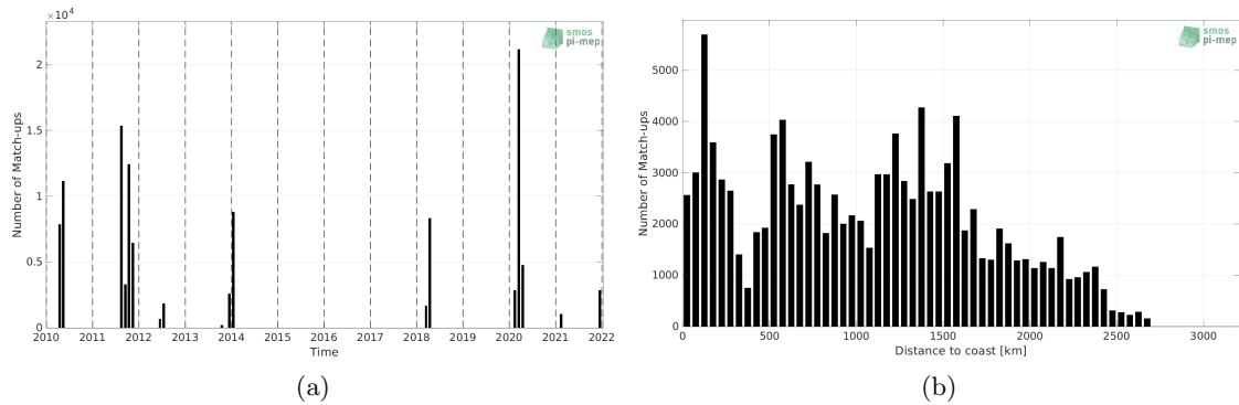
Figure 1: Number of match-ups between TSG (SAMOS) and SMOS SSS L4 v1 - Monthly (CMEMS-CNR) SSS as a function of time (a) and as function of the distance to coast (b) over the South Atlantic Ocean Pi-MEP region and for the full satellite product period.
