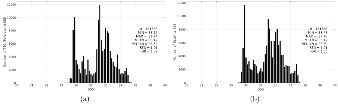
Figure 3: Histograms of SSS from TSG (Polarstern) (a) and SMOS SSS L4 v1 - Monthly (CMEMS-CNR) (b) considering all match-up pairs per bins of 0.1 over the South Atlantic Ocean Pi-MEP region and for the full satellite product period.
