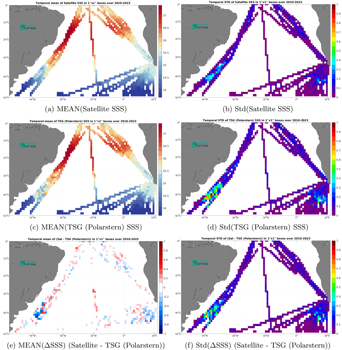
Figure 7: Temporal mean (left) and Std (right) of SSS from SMOS SSS L4 v1 - Monthly (CMEMS-CNR) (top), TSG (Polarstern) (middle), and of \Delta SSS (Satellite - TSG (Polarstern)). Only match-up pairs are used to generate these maps.
