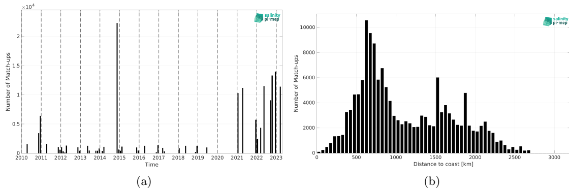
Figure 2: Number of match-ups between TSG (Polarstern) and SMOS SSS L4 v1 - Monthly (CMEMS-CNR) SSS as a function of time (a) and as function of the distance to coast (b) over the South Atlantic Ocean Pi-MEP region and for the full satellite product period.
