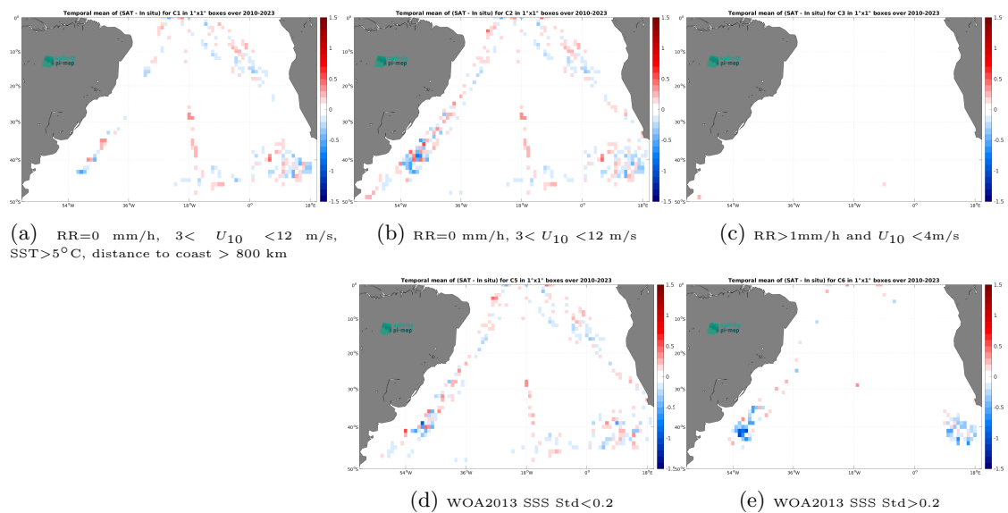
Figure 14: Temporal mean gridded over spatial boxes of size 1^\circ \times 1^\circ of \Delta SSS (SMOS SSS L4 v1 - Monthly (CMEMS-CNR) - TSG (Polarstern)) for 5 different subdatasets corresponding to:RR=0 mm/h, 3 < U_{10} < 12 m/s, SST >5^\circ\text{C} , distance to coast > 800 km (a), RR=0 mm/h, 3 < U_{10} < 12 m/s (b), RR >1 mm/h and U_{10} < 4 m/s (c), WOA2013 SSS Std <0.2 (d), WOA2013 SSS Std >0.2 (e).
