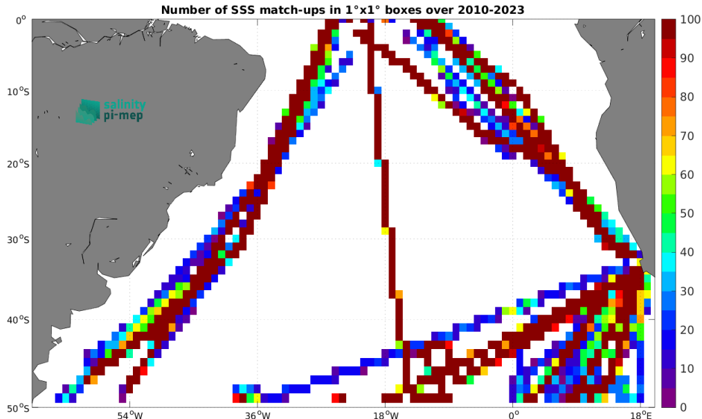
Figure 5: Number of SSS match-ups between TSG (Polarstern) SSS and the SMOS SSS L4 v1 - Monthly (CMEMS-CNR) SSS product for the South Atlantic Ocean Pi-MEP region over 1^\circ \times 1^\circ boxes and for the full satellite product period.
