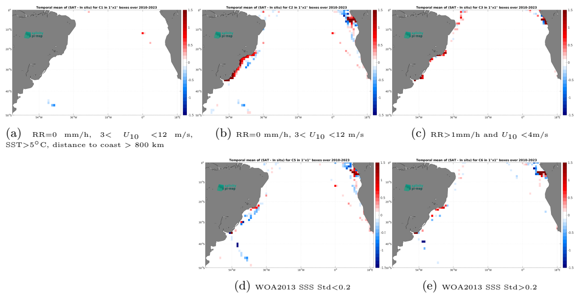
Figure 14: Temporal mean gridded over spatial boxes of size 1^\circ \times 1^\circ of \Delta SSS (SMOS SSS L4 v1 - Monthly (CMEMS-CNR) - TSG (LEGOS-DM)) for 5 different subdatasets corresponding to:RR=0 mm/h, 3 < U_{10} < 12 m/s, SST >5^\circ\text{C} , distance to coast > 800 km (a), RR=0 mm/h, 3 < U_{10} < 12 m/s (b), RR >1 mm/h and U_{10} < 4 m/s (c), WOA2013 SSS Std <0.2 (d), WOA2013 SSS Std >0.2 (e).
