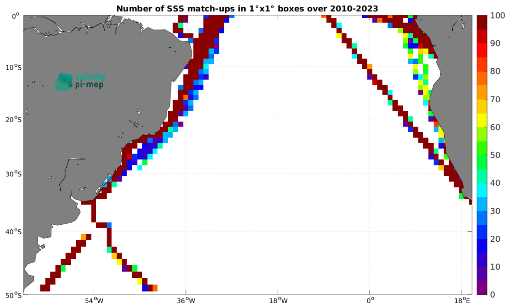
Figure 5: Number of SSS match-ups between TSG (LEGOS-DM) SSS and the SMOS SSS L4 v1 - Monthly (CMEMS-CNR) SSS product for the South Atlantic Ocean Pi-MEP region over 1^\circ \times 1^\circ boxes and for the full satellite product period.
