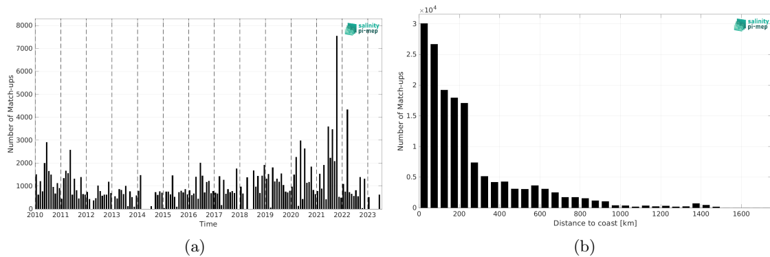
Figure 2: Number of match-ups between TSG (LEGOS-DM) and SMOS SSS L4 v1 - Monthly (CMEMS-CNR) SSS as a function of time (a) and as function of the distance to coast (b) over the South Atlantic Ocean Pi-MEP region and for the full satellite product period.
