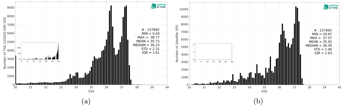
Figure 3: Histograms of SSS from TSG (LEGOS-DM) (a) and SMOS SSS L4 v1 - Monthly (CMEMS-CNR) (b) considering all match-up pairs per bins of 0.1 over the South Atlantic Ocean Pi-MEP region and for the full satellite product period.
