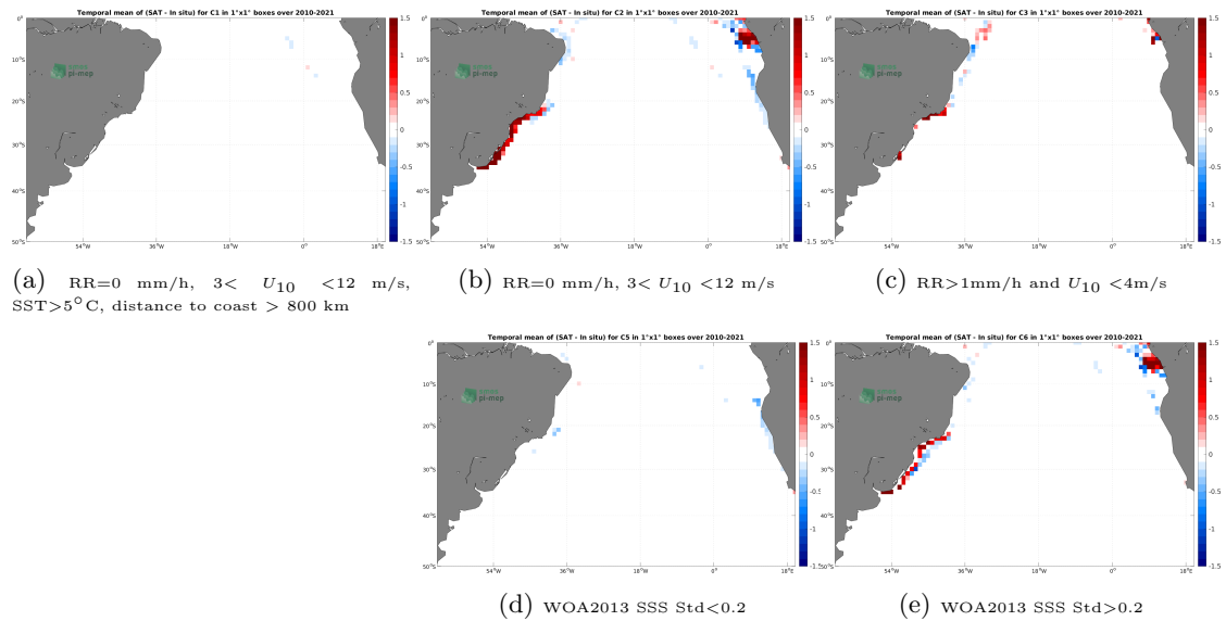
Figure 12: Temporal mean gridded over spatial boxes of size 1^\circ \times 1^\circ of \Delta SSS (SMOS SSS L4 v1 - Monthly (CMEMS-CNR) - TSG (LEGOS-DM)) for 5 different subdatasets corresponding to:RR=0 mm/h, 3 < U_{10} < 12 m/s, SST >5^\circ\text{C} , distance to coast > 800 km (a), RR=0 mm/h, 3 < U_{10} < 12 m/s (b), RR >1 mm/h and U_{10} < 4 m/s (c), WOA2013 SSS Std <0.2 (d), WOA2013 SSS Std >0.2 (e).
