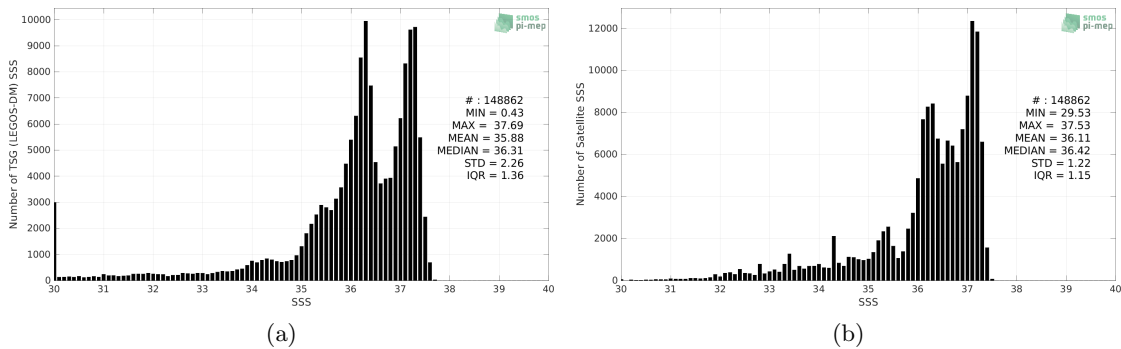
Figure 2: Histograms of SSS from TSG (LEGOS-DM) (a) and SMOS SSS L4 v1 - Monthly (CMEMS-CNR) (b) considering all match-up pairs per bins of 0.1 over the South Atlantic Ocean Pi-MEP region and for the full satellite product period.
