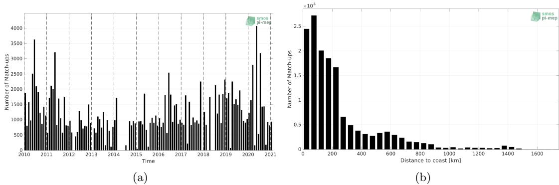
Figure 1: Number of match-ups between TSG (LEGOS-DM) and SMOS SSS L4 v1 - Monthly (CMEMS-CNR) SSS as a function of time (a) and as function of the distance to coast (b) over the South Atlantic Ocean Pi-MEP region and for the full satellite product period.
