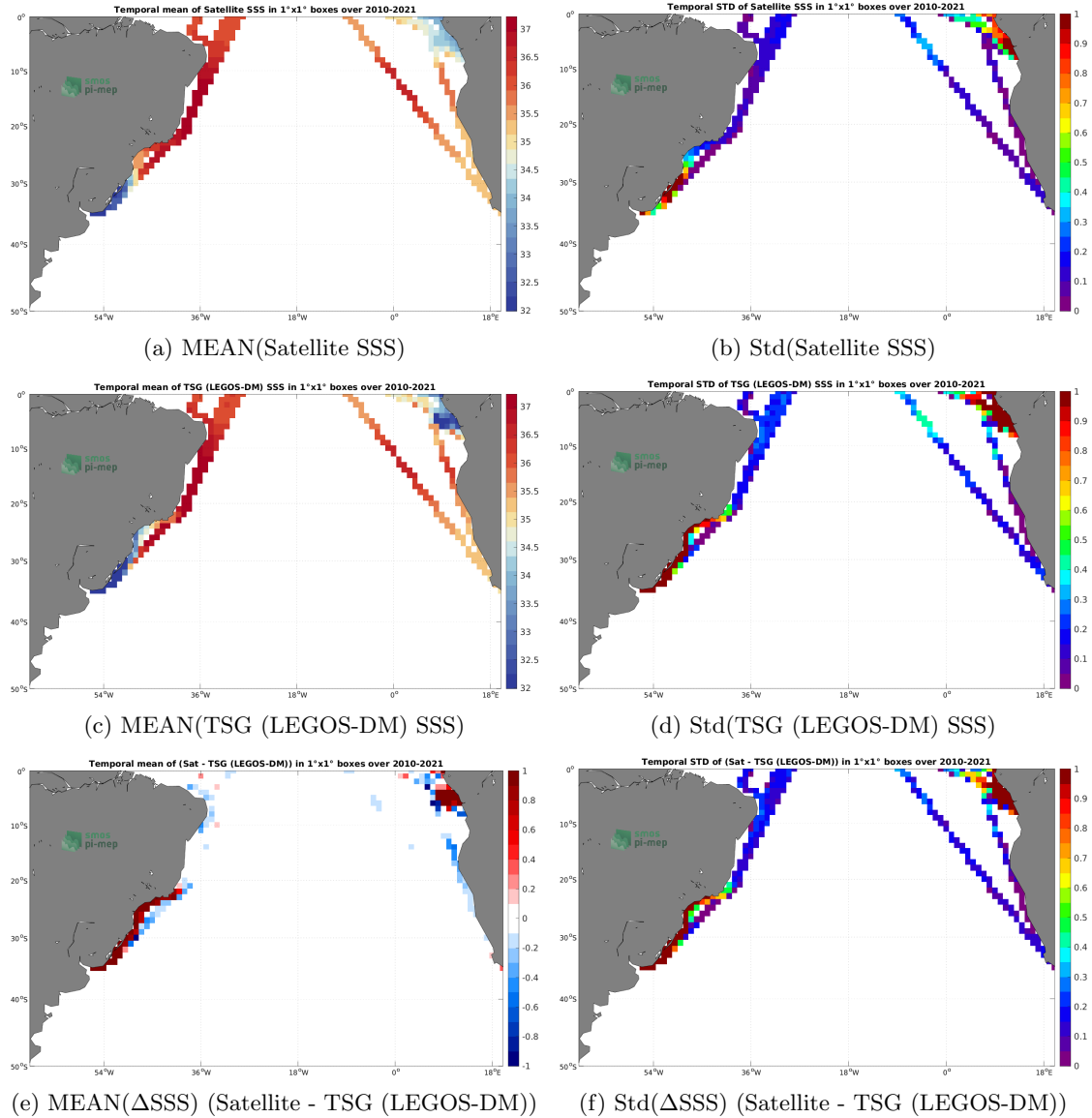
Figure 6: Temporal mean (left) and Std (right) of SSS from SMOS SSS L4 v1 - Monthly (CMEMS-CNR) (top), TSG (LEGOS-DM) (middle), and of \Delta SSS (Satellite - TSG (LEGOS-DM)). Only match-up pairs are used to generate these maps.
