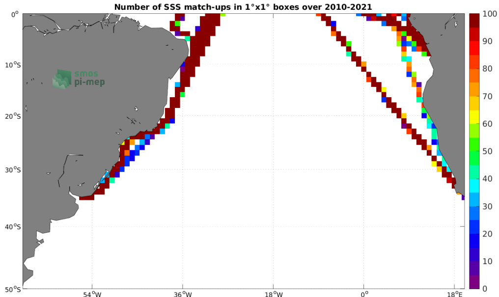
Figure 4: Number of SSS match-ups between TSG (LEGOS-DM) SSS and the SMOS SSS L4 v1 - Monthly (CMEMS-CNR) SSS product for the South Atlantic Ocean Pi-MEP region over 1^\circ \times 1^\circ boxes and for the full satellite product period.
