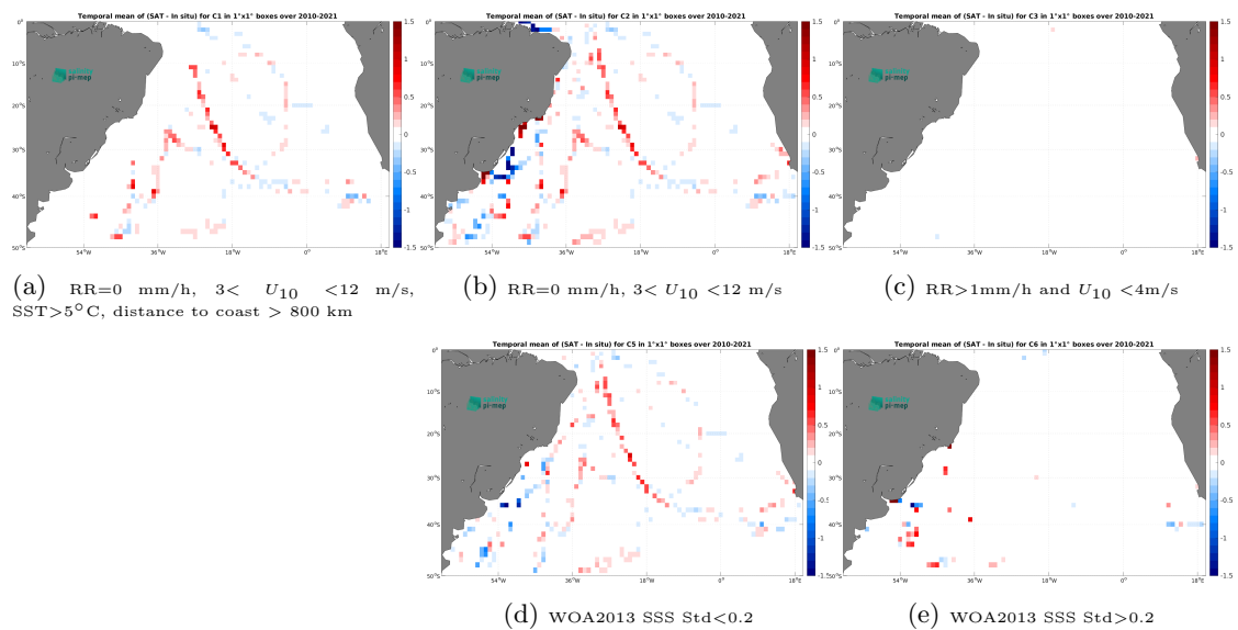
Figure 14: Temporal mean gridded over spatial boxes of size 1^\circ \times 1^\circ of \Delta\text{SSS} (SMOS SSS L4 v1 - Monthly (CMEMS-CNR) - TSG (GOSUD-Sailing-ship)) for 5 different subdatasets corresponding to:RR=0 mm/h, 3 < U_{10} < 12 m/s, SST >5^\circ\text{C} , distance to coast > 800 km (a), RR=0 mm/h, 3 < U_{10} < 12 m/s (b), RR >1 mm/h and U_{10} < 4 m/s (c), WOA2013 SSS Std <0.2 (d), WOA2013 SSS Std >0.2 (e).
