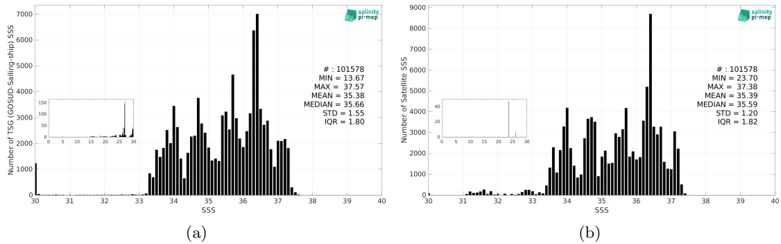
Figure 3: Histograms of SSS from TSG (GOSUD-Sailing-ship) (a) and SMOS SSS L4 v1 - Monthly (CMEMS-CNR) (b) considering all match-up pairs per bins of 0.1 over the South Atlantic Ocean Pi-MEP region and for the full satellite product period.
