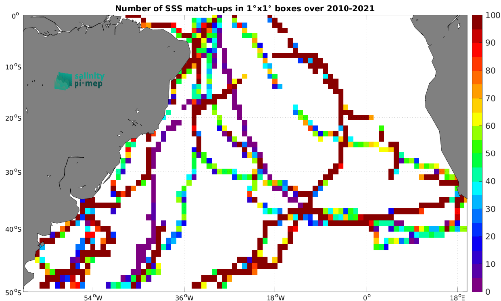
Figure 5: Number of SSS match-ups between TSG (GOSUD-Sailing-ship) SSS and the SMOS SSS L4 v1 - Monthly (CMEMS-CNR) SSS product for the South Atlantic Ocean Pi-MEP region over 1^\circ \times 1^\circ boxes and for the full satellite product period.
