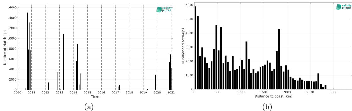
Figure 2: Number of match-ups between TSG (GOSUD-Sailing-ship) and SMOS SSS L4 v1 - Monthly (CMEMS-CNR) SSS as a function of time (a) and as function of the distance to coast (b) over the South Atlantic Ocean Pi-MEP region and for the full satellite product period.
