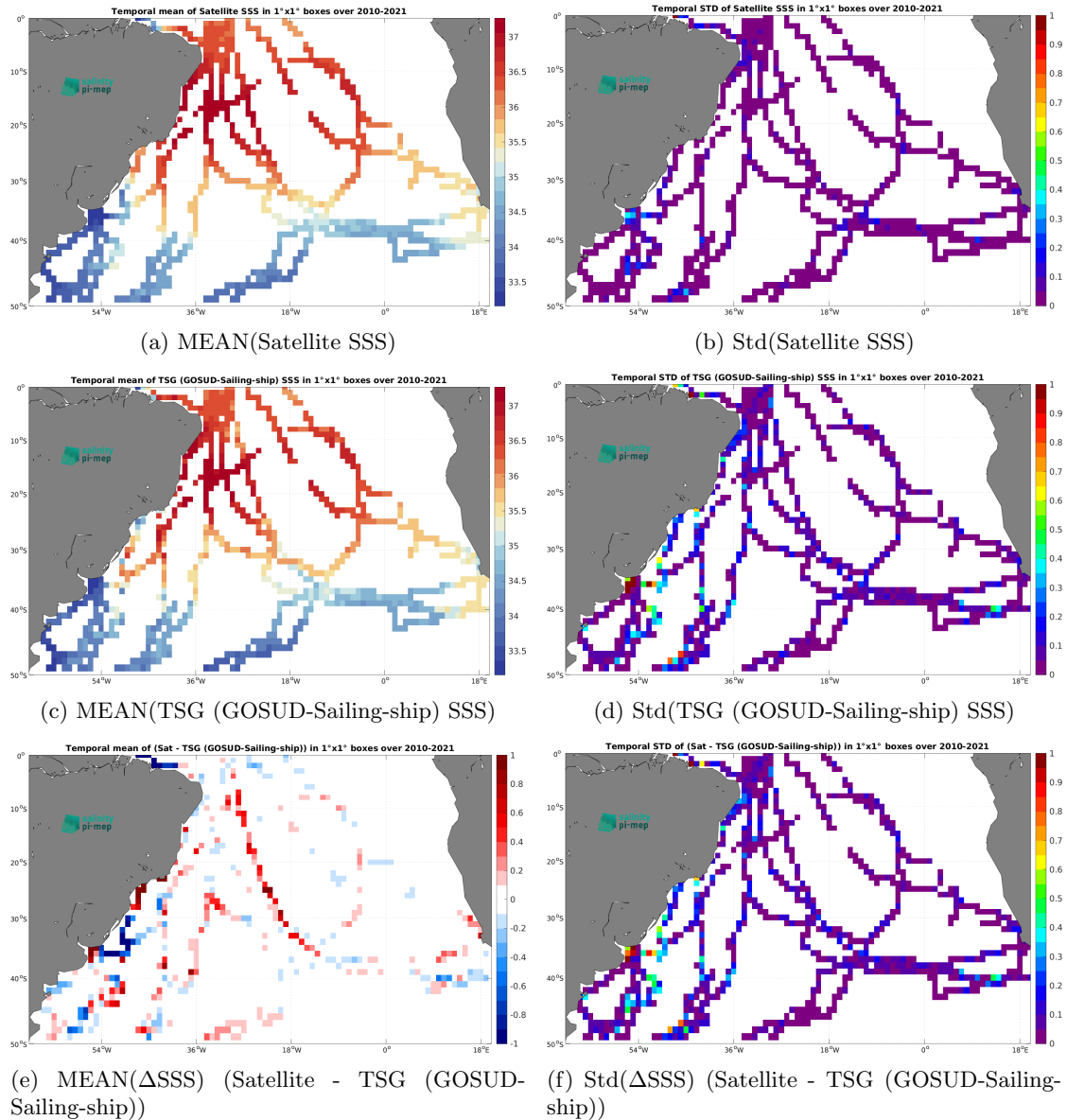
Figure 7: Temporal mean (left) and Std (right) of SSS from SMOS SSS L4 v1 - Monthly (CMEMS-CNR) (top), TSG (GOSUD-Sailing-ship) (middle), and of \Delta SSS (Satellite - TSG (GOSUD-Sailing-ship)). Only match-up pairs are used to generate these maps.
