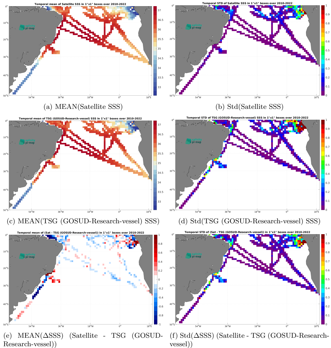
Figure 7: Temporal mean (left) and Std (right) of SSS from SMOS SSS L4 v1 - Monthly (CMEMS-CNR) (top), TSG (GOSUD-Research-vessel) (middle), and of \Delta SSS (Satellite - TSG (GOSUD-Research-vessel)). Only match-up pairs are used to generate these maps.
