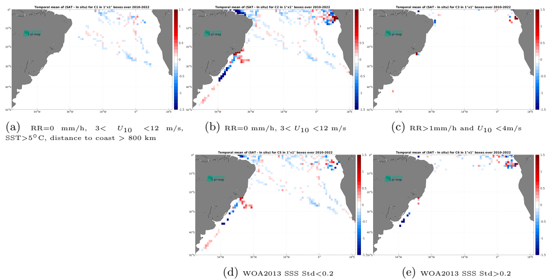
Figure 14: Temporal mean gridded over spatial boxes of size 1^\circ \times 1^\circ of \Delta SSS (SMOS SSS L4 v1 - Monthly (CMEMS-CNR) - TSG (GOSUD-Research-vessel)) for 5 different subdatasets corresponding to:RR=0 mm/h, 3 < U_{10} < 12 m/s, SST >5^\circ\text{C} , distance to coast > 800 km (a), RR=0 mm/h, 3 < U_{10} < 12 m/s (b), RR >1 mm/h and U_{10} < 4 m/s (c), WOA2013 SSS Std <0.2 (d), WOA2013 SSS Std >0.2 (e).
