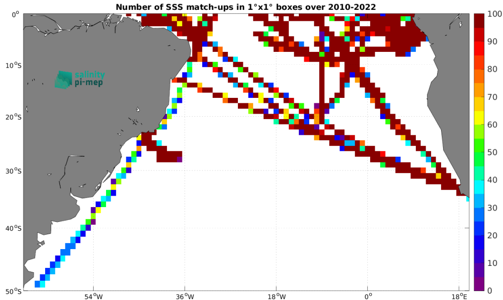
Figure 5: Number of SSS match-ups between TSG (GOSUD-Research-vessel) SSS and the SMOS SSS L4 v1 - Monthly (CMEMS-CNR) SSS product for the South Atlantic Ocean Pi-MEP region over 1^\circ \times 1^\circ boxes and for the full satellite product period.
