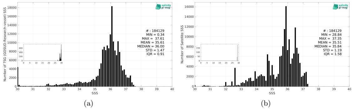
Figure 3: Histograms of SSS from TSG (GOSUD-Research-vessel) (a) and SMOS SSS L4 v1 - Monthly (CMEMS-CNR) (b) considering all match-up pairs per bins of 0.1 over the South Atlantic Ocean Pi-MEP region and for the full satellite product period.
