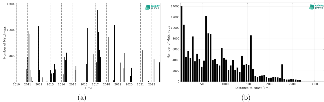
Figure 2: Number of match-ups between TSG (GOSUD-Research-vessel) and SMOS SSS L4 v1 - Monthly (CMEMS-CNR) SSS as a function of time (a) and as function of the distance to coast (b) over the South Atlantic Ocean Pi-MEP region and for the full satellite product period.
