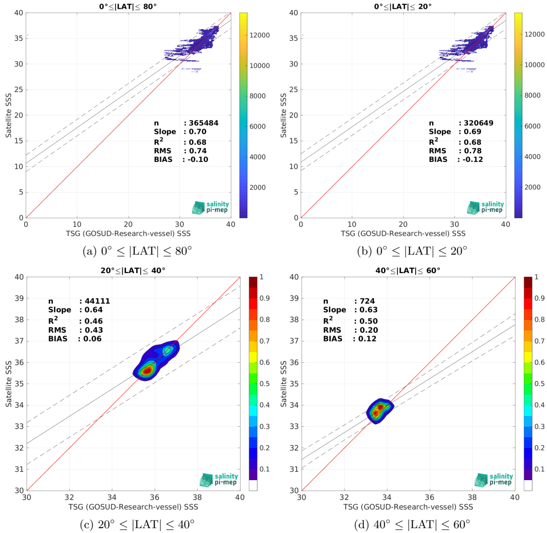
Figure 9: Contour maps of the concentration of SMOS SSS L4 v1 - Monthly (CMEMS-CNR) SSS (y-axis) versus TSG (GOSUD-Research-vessel) SSS (x-axis) at match-up pairs for different latitude bands. For each plot, the red line shows x=y . The black thin and dashed lines indicate a linear fit through the data cloud and the \pm 95\% confidence levels, respectively. The number match-up pairs n , the slope and R^2 coefficient of the linear fit, the root mean square (RMS) and the mean bias between satellite and in situ data are indicated for each latitude band in each plots.
