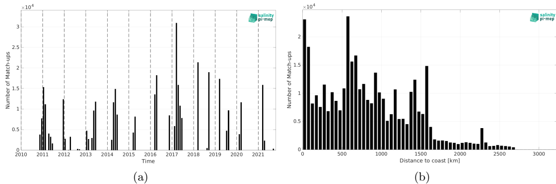
Figure 1: Number of match-ups between TSG (GOSUD-Research-vessel) and SMOS SSS L4 v1 - Monthly (CMEMS-CNR) SSS as a function of time (a) and as function of the distance to coast (b) over the South Atlantic Ocean Pi-MEP region and for the full satellite product period.
