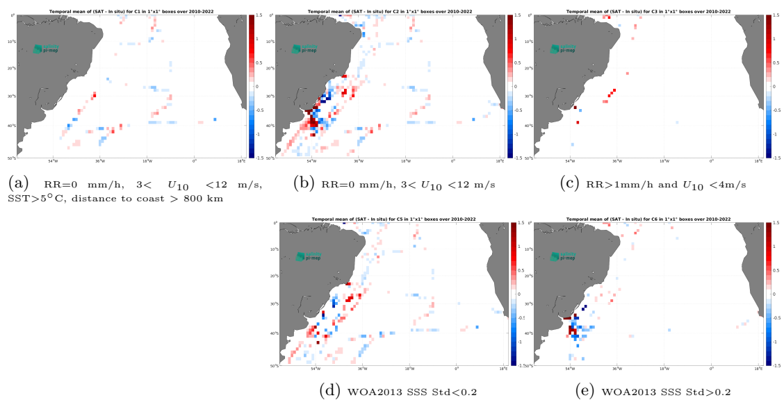
Figure 14: Temporal mean gridded over spatial boxes of size 1^\circ \times 1^\circ of \Delta SSS (SMOS SSS L4 v1 - Monthly (CMEMS-CNR) - TSG (CSIC-UTM)) for 5 different subdatasets corresponding to:RR=0 mm/h, 3 < U_{10} < 12 m/s, SST >5^\circ\text{C} , distance to coast > 800 km (a), RR=0 mm/h, 3 < U_{10} < 12 m/s (b), RR >1 mm/h and U_{10} < 4 m/s (c), WOA2013 SSS Std <0.2 (d), WOA2013 SSS Std >0.2 (e).
