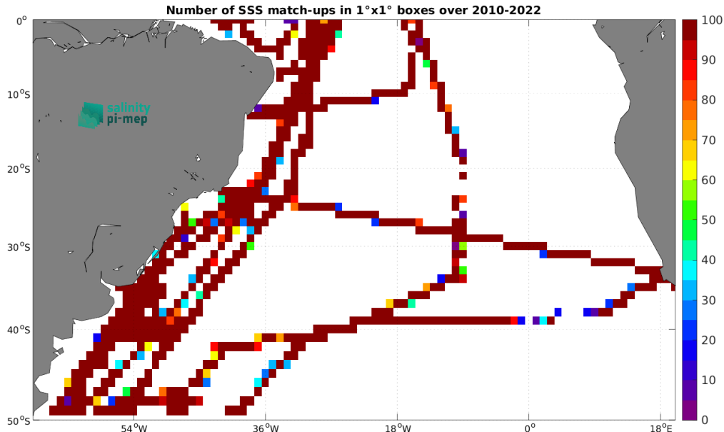
Figure 5: Number of SSS match-ups between TSG (CSIC-UTM) SSS and the SMOS SSS L4 v1 - Monthly (CMEMS-CNR) SSS product for the South Atlantic Ocean Pi-MEP region over 1^\circ \times 1^\circ boxes and for the full satellite product period.
