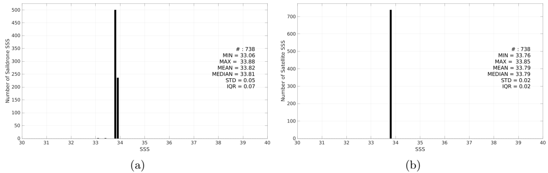
Figure 3: Histograms of SSS from Saildrone (a) and SMOS SSS L4 v1 - Monthly (CMEMS-CNR) (b) considering all match-up pairs per bins of 0.1 over the South Atlantic Ocean Pi-MEP region and for the full satellite product period.
