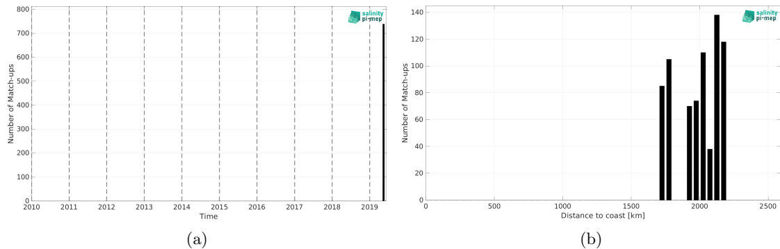
Figure 2: Number of match-ups between Saildrone and SMOS SSS L4 v1 - Monthly (CMEMS-CNR) SSS as a function of time (a) and as function of the distance to coast (b) over the South Atlantic Ocean Pi-MEP region and for the full satellite product period.
