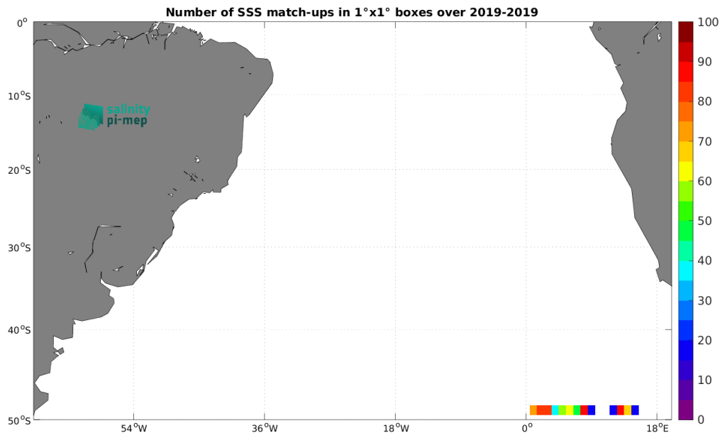
Figure 5: Number of SSS match-ups between Sailability SSS and the SMOS SSS L4 v1 - Monthly (CMEMS-CNR) SSS product for the South Atlantic Ocean Pi-MEP region over 1^\circ \times 1^\circ boxes and for the full satellite product period.
