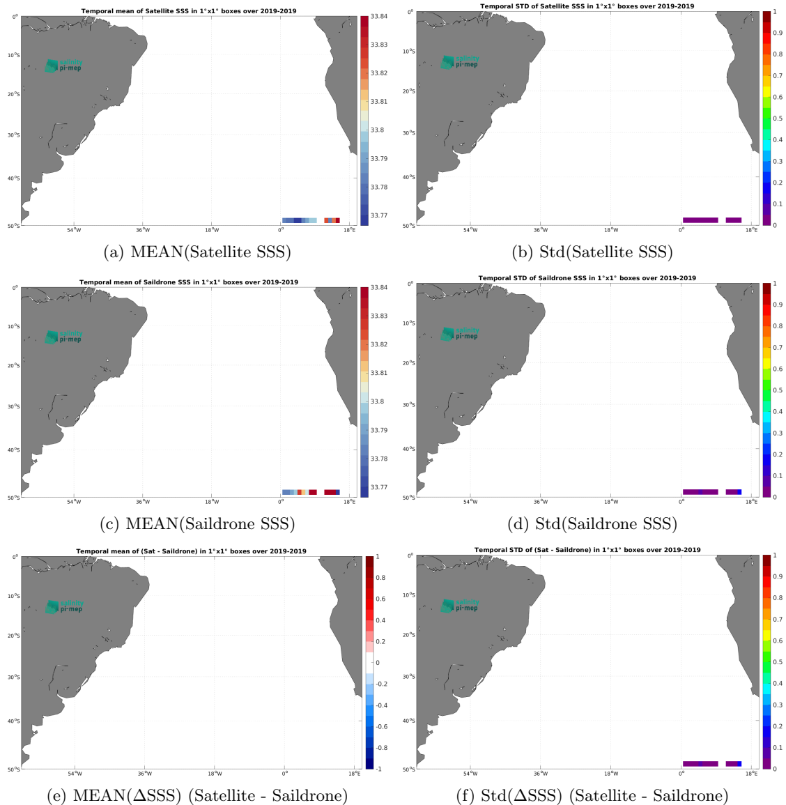
Figure 7: Temporal mean (left) and Std (right) of SSS from SMOS SSS L4 v1 - Monthly (CMEMS-CNR) (top), Saildrone (middle), and of \Delta SSS (Satellite - Saildrone). Only match-up pairs are used to generate these maps.
