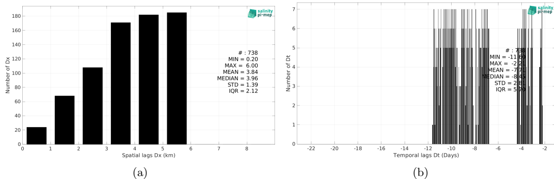
Figure 6: Histograms of the spatial (a) and temporal (b) lags between the location/time of the Sairdrone measurement and the date of the corresponding SMOS SSS L4 v1 - Monthly (CMEMS-CNR) SSS pixel.
