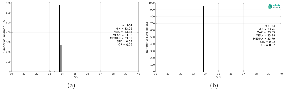
Figure 2: Histograms of SSS from Saildrone (a) and SMOS SSS L4 v1 - Monthly (CMEMS-CNR) (b) considering all match-up pairs per bins of 0.1 over the South Atlantic Ocean Pi-MEP region and for the full satellite product period.
