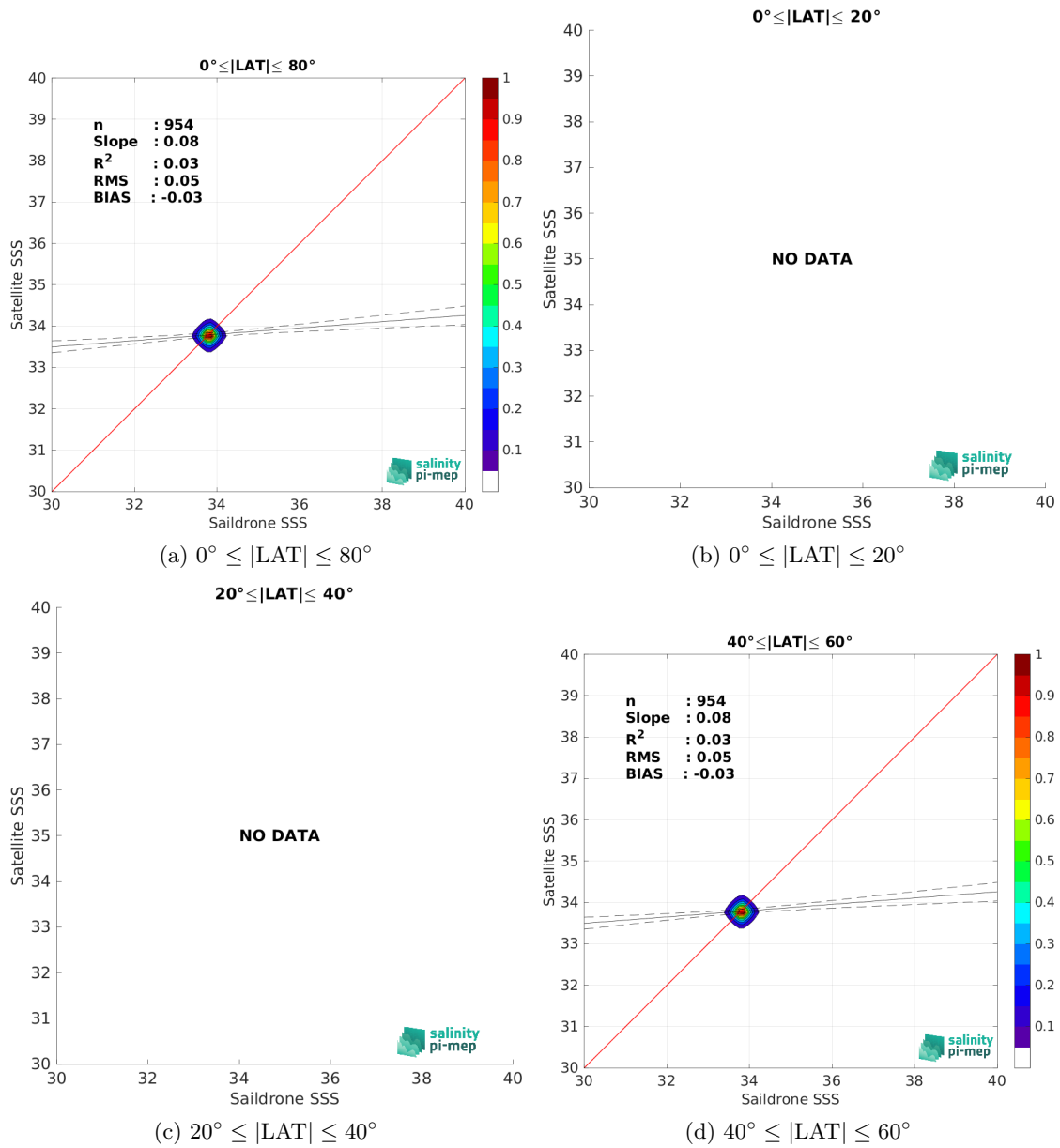
Figure 9: Contour maps of the concentration of SMOS SSS L4 v1 - Monthly (CMEMS-CNR) SSS (y-axis) versus Saildrone SSS (x-axis) at match-up pairs for different latitude bands. For each plot, the red line shows x=y . The black thin and dashed lines indicate a linear fit through the data cloud and the \pm 95\% confidence levels, respectively. The number match-up pairs n , the slope and R^2 coefficient of the linear fit, the root mean square (RMS) and the mean bias between satellite and in situ data are indicated for each latitude band in each plots.
