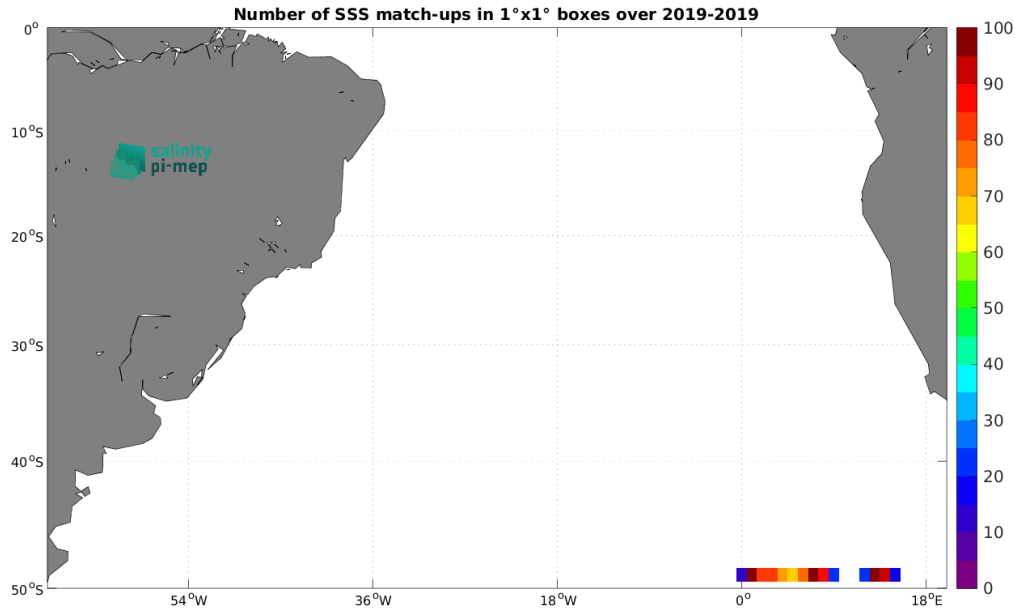
Figure 4: Number of SSS match-ups between Saildrone SSS and the SMOS SSS L4 v1 - Monthly (CMEMS-CNR) SSS product for the South Atlantic Ocean Pi-MEP region over 1^\circ \times 1^\circ boxes and for the full satellite product period.
