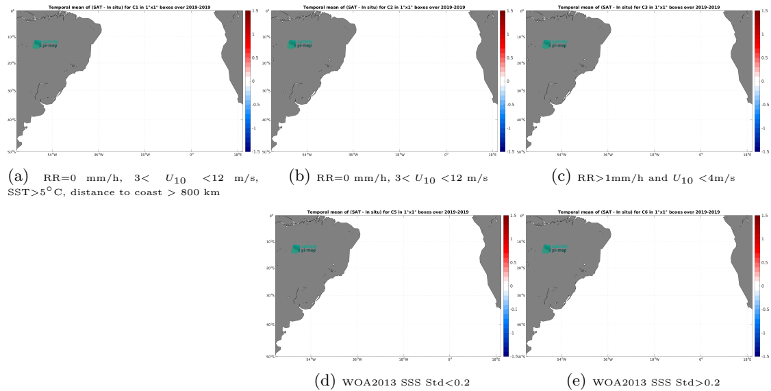
Figure 12: Temporal mean gridded over spatial boxes of size 1^{\circ}\times 1^{\circ} of \Delta\text{SSS} (SMOS SSS L4 v1 - Monthly (CMEMS-CNR) - Saildrone) for 5 different subdatasets corresponding to:RR=0 mm/h, 3 < U_{10} < 12 m/s, SST >5^{\circ}\text{C} , distance to coast > 800 km (a), RR=0 mm/h, 3 < U_{10} < 12 m/s (b), RR >1 mm/h and U_{10} < 4 m/s (c), WOA2013 SSS Std <0.2 (d), WOA2013 SSS Std >0.2 (e).
