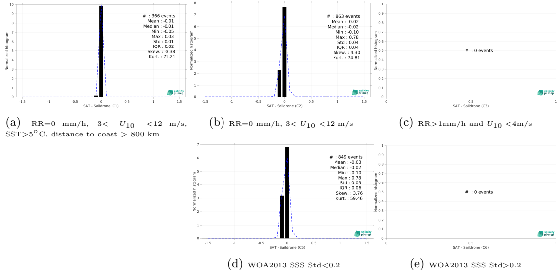
Figure 13: Normalized histogram of \Delta SSS (SMOS SSS L4 v1 - Monthly (CMEMS-CNR) - Saildrone) for 5 different subdatasets corresponding to: RR=0 mm/h, 3 < U_{10} < 12 m/s, SST>5°C, distance to coast > 800 km (a), RR=0 mm/h, 3 < U_{10} < 12 m/s (b), RR>1mm/h and U_{10} < 4 m/s (c), WOA2013 SSS Std<0.2 (d), WOA2013 SSS Std>0.2 (e).
