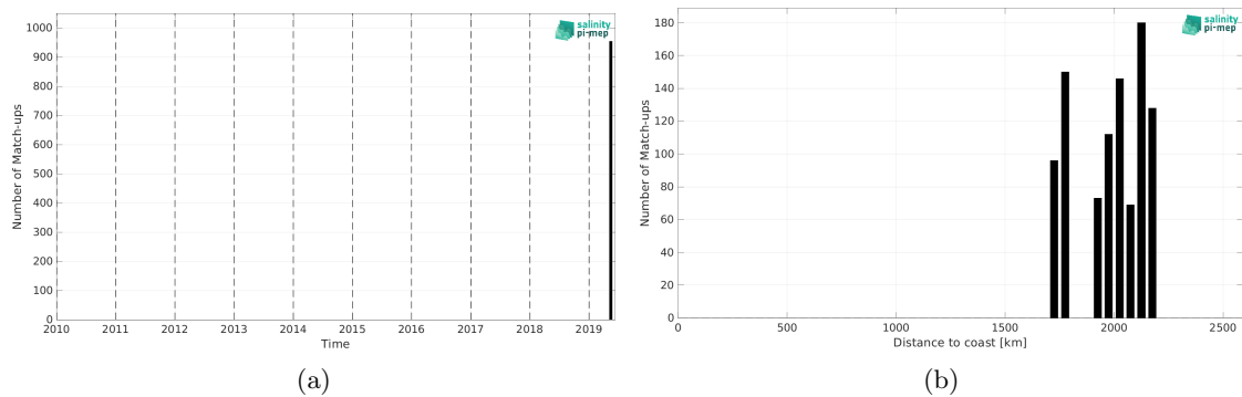
Figure 1: Number of match-ups between Saildrone and SMOS SSS L4 v1 - Monthly (CMEMS-CNR) SSS as a function of time (a) and as function of the distance to coast (b) over the South Atlantic Ocean Pi-MEP region and for the full satellite product period.
