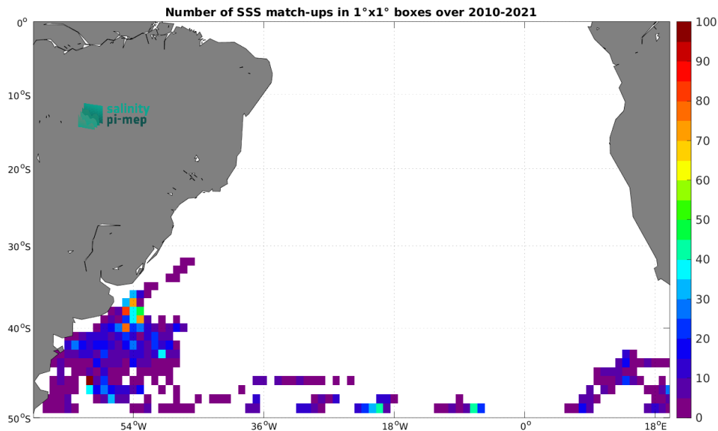
Figure 5: Number of SSS match-ups between Marine mammals SSS and the SMOS SSS L4 v1 - Monthly (CMEMS-CNR) SSS product for the South Atlantic Ocean Pi-MEP region over 1^\circ \times 1^\circ boxes and for the full satellite product period.
