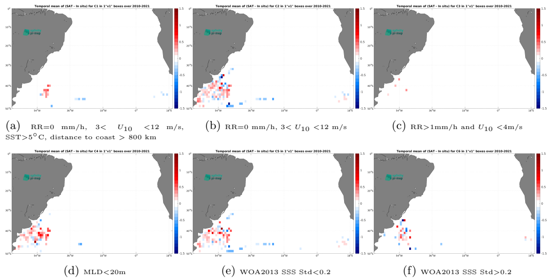
Figure 14: Temporal mean gridded over spatial boxes of size 1^\circ \times 1^\circ of \Delta SSS (SMOS SSS L4 v1 - Monthly (CMEMS-CNR) - Marine mammals) for 6 different subdatasets corresponding to:RR=0 mm/h, 3 < U_{10} < 12 m/s, SST > 5^\circ\text{C} , distance to coast > 800 km (a), RR=0 mm/h, 3 < U_{10} < 12 m/s (b), RR > 1 mm/h and U_{10} < 4 m/s (c),MLD < 20 m (d),WOA2013 SSS Std < 0.2 (e),WOA2013 SSS Std > 0.2 (f).
