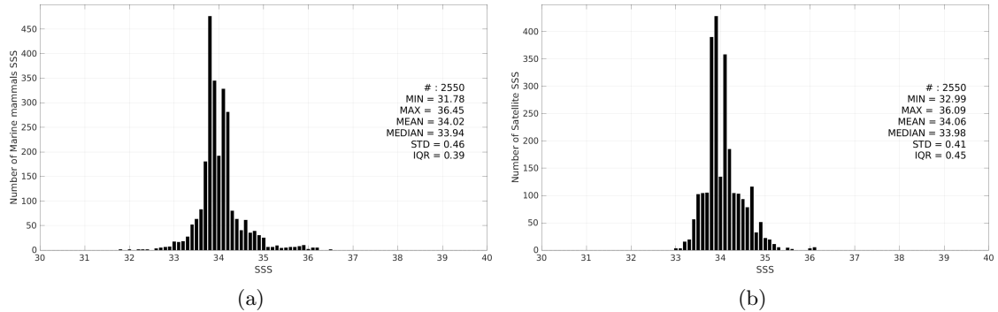
Figure 3: Histograms of SSS from Marine mammals (a) and SMOS SSS L4 v1 - Monthly (CMEMS-CNR) (b) considering all match-up pairs per bins of 0.1 over the South Atlantic Ocean Pi-MEP region and for the full satellite product period.
