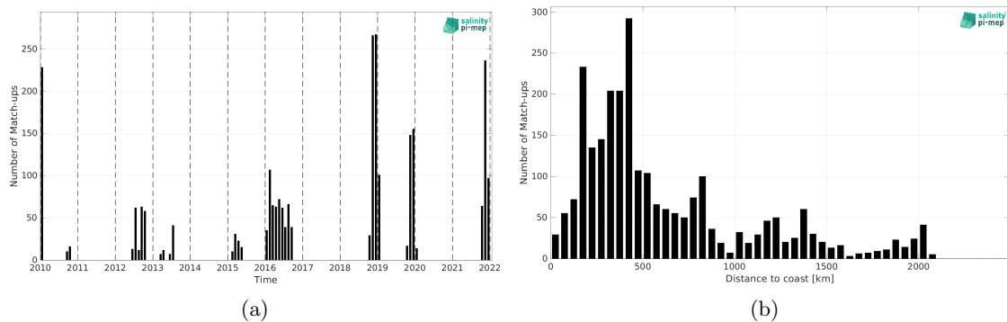
Figure 2: Number of match-ups between Marine mammals and SMOS SSS L4 v1 - Monthly (CMEMS-CNR) SSS as a function of time (a) and as function of the distance to coast (b) over the South Atlantic Ocean Pi-MEP region and for the full satellite product period.
