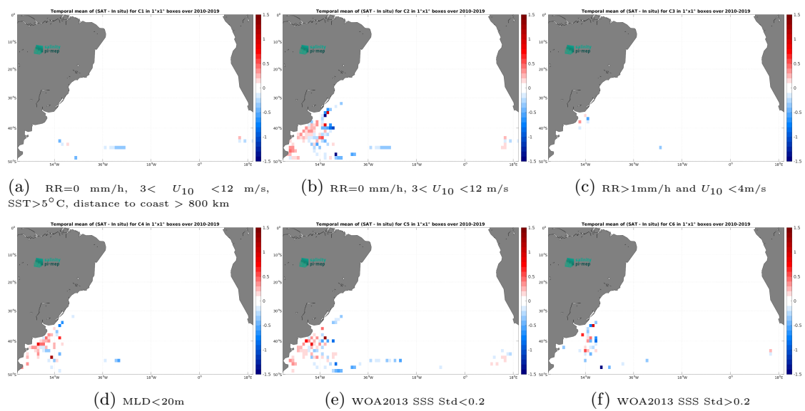
Figure 12: Temporal mean gridded over spatial boxes of size 1^\circ \times 1^\circ of \Delta SSS (SMOS SSS L4 v1 - Monthly (CMEMS-CNR) - Marine mammals) for 6 different subdatasets corresponding to: RR=0 mm/h, 3 < U_{10} < 12 m/s, SST > 5^\circ C , distance to coast > 800 km (a), RR=0 mm/h, 3 < U_{10} < 12 m/s (b), RR > 1 mm/h and U_{10} < 4 m/s (c), MLD < 20 m (d), WOA2013 SSS Std < 0.2 (e), WOA2013 SSS Std > 0.2 (f).
